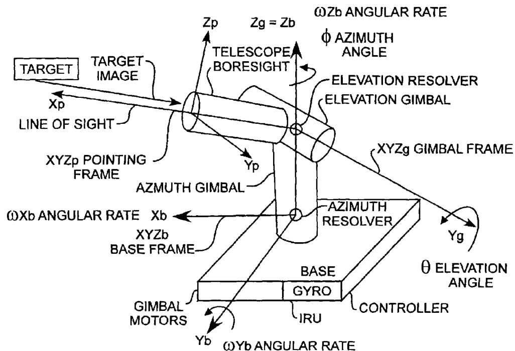
OFF-GIMBAL CONFIGURATION
