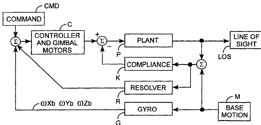
OFF-GIMBAL CONTROL SYSTEM (PRIOR ART)
