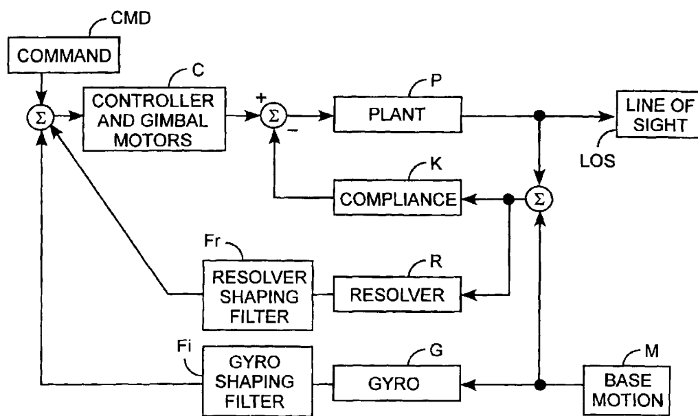
OFF-GIMBAL CONTROL SYSTEM (NEW) FIG. 3
