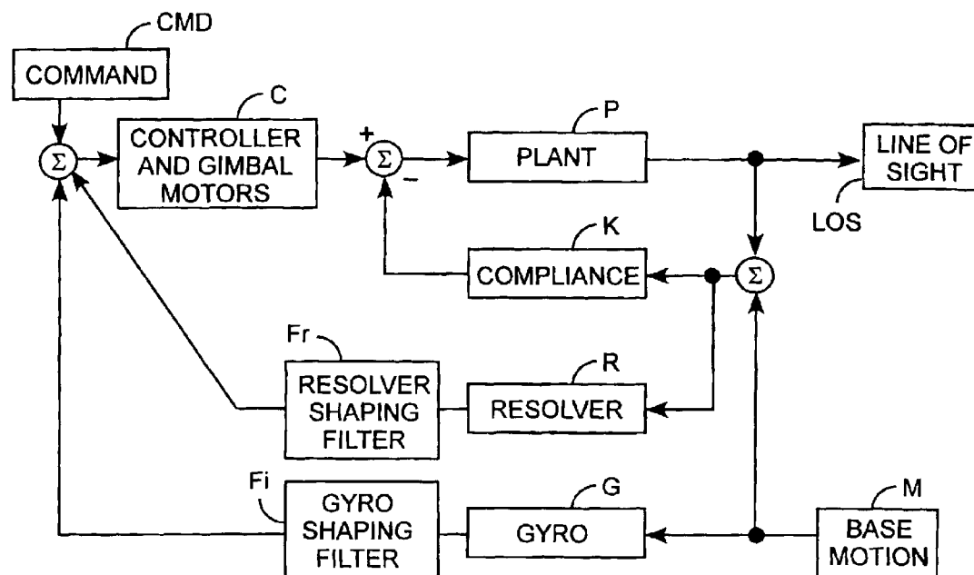
OFF-GIMBAL CONTROL SYSTEM (NEW)
