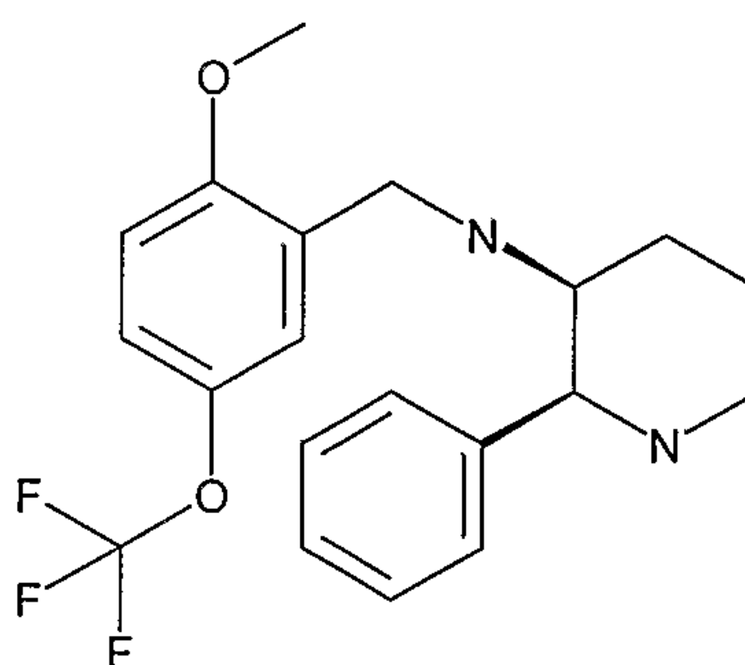
Formula 2 (2S,3S)(2-Methoxy-5-trifluoromethoxy-benzyl)-(2-phenyl-piperidin-3-yl)-amine)
