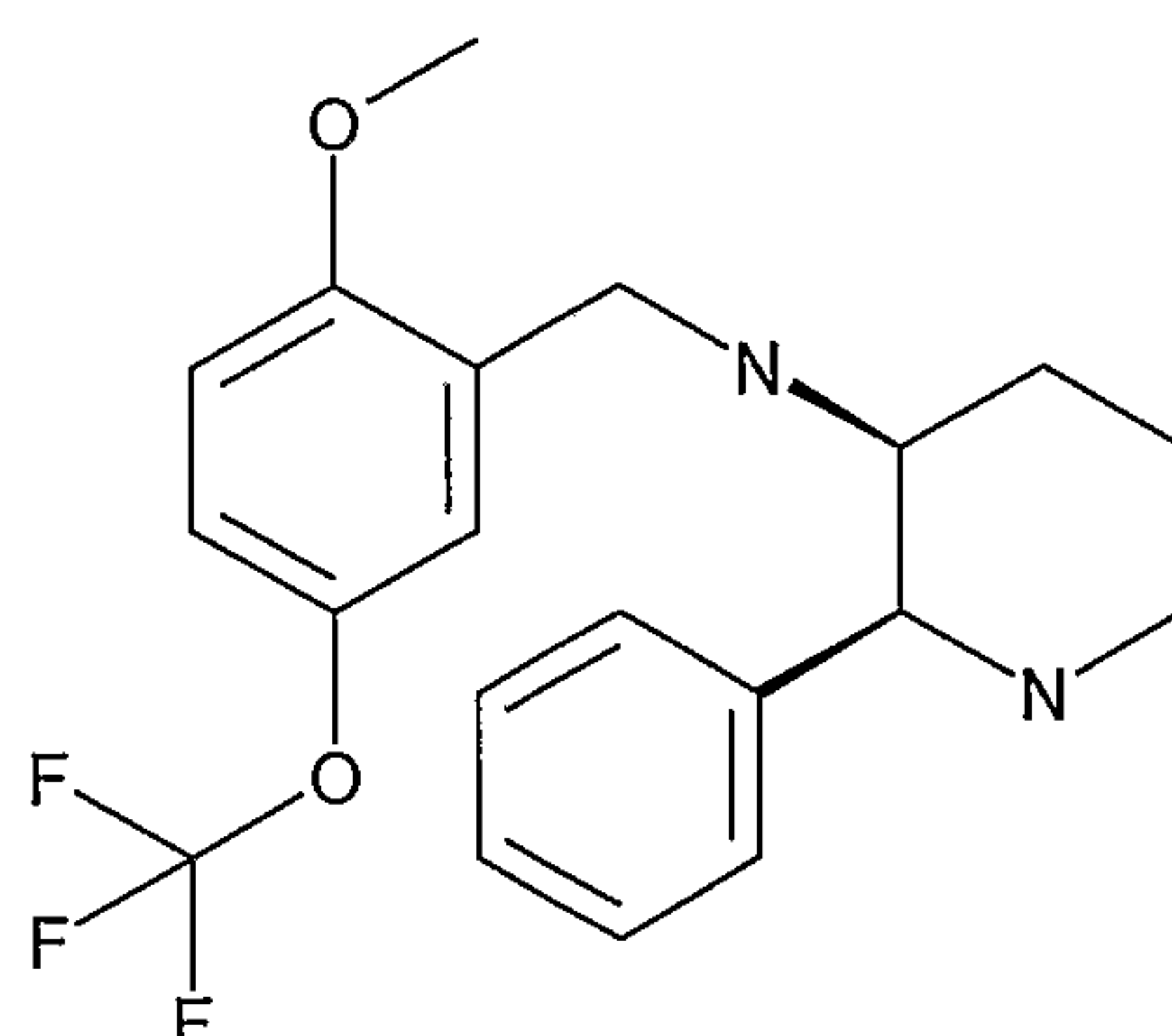
Formula 2
