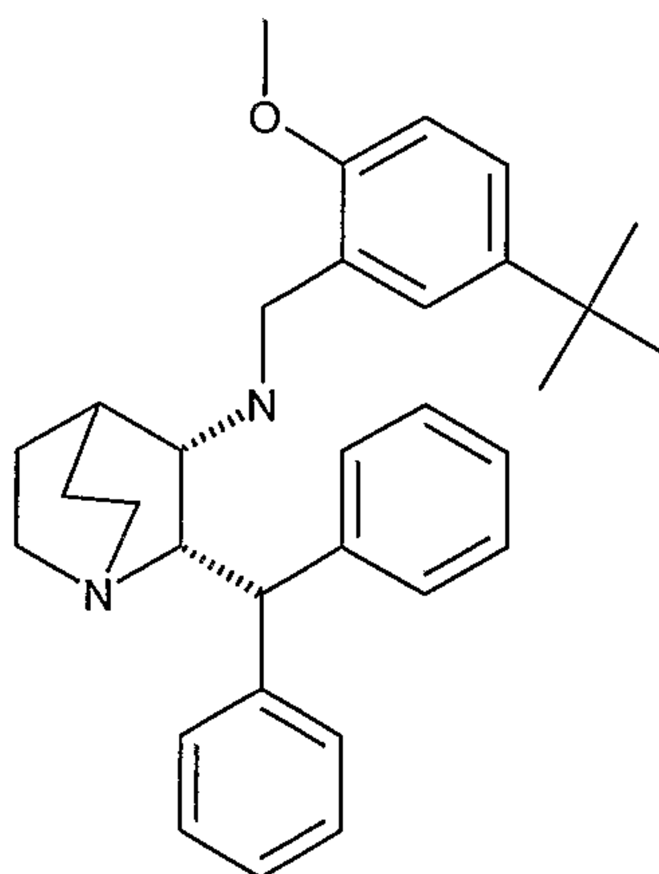
Formula 1 (2S,3S) (2-Benzhydryl-1-aza-bicyclo[2.2.2]oct-3-yl)-(5-tert-butyl-2-methoxy-benzyl)-amine
