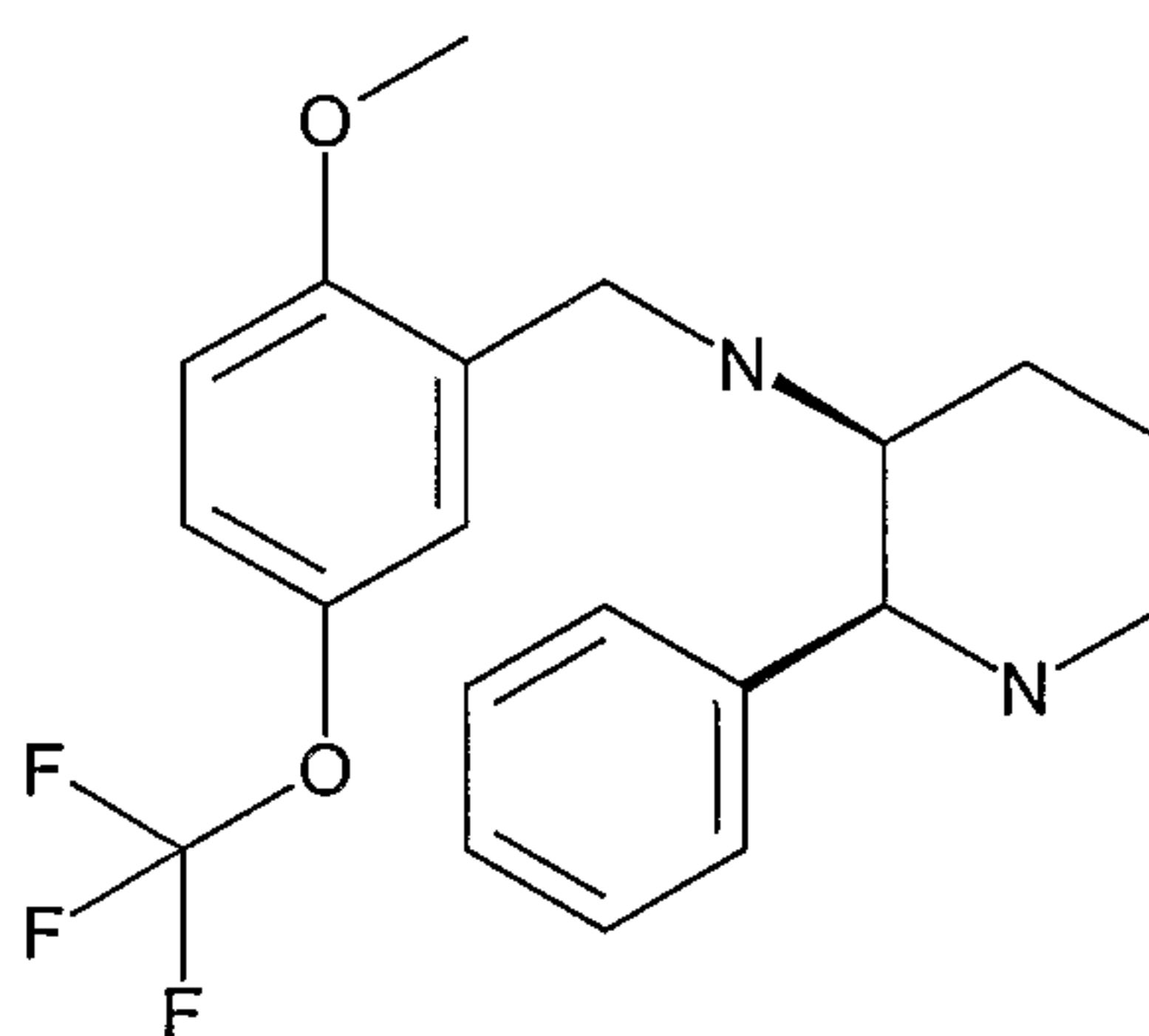
Formula 2
