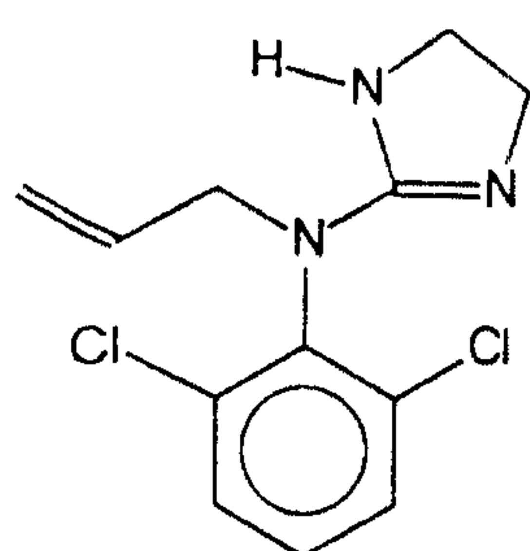
Alinidine
