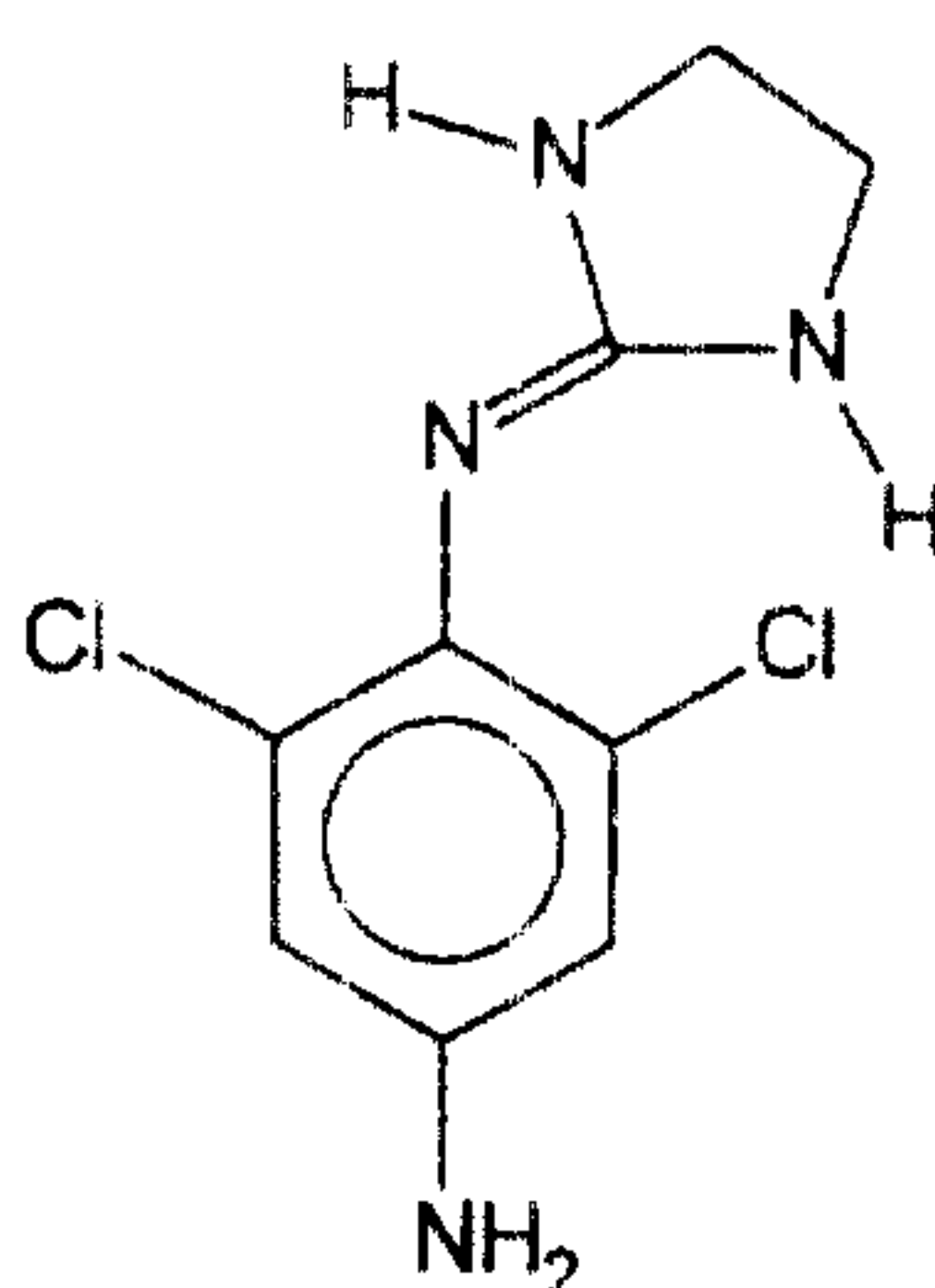
Iopidine
