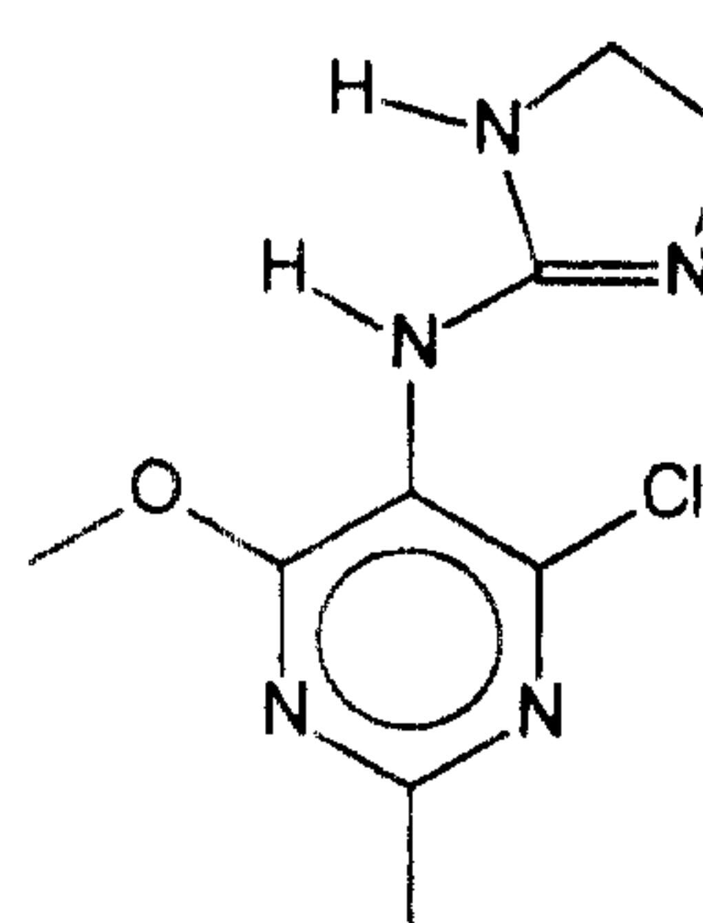
Moxonidine
