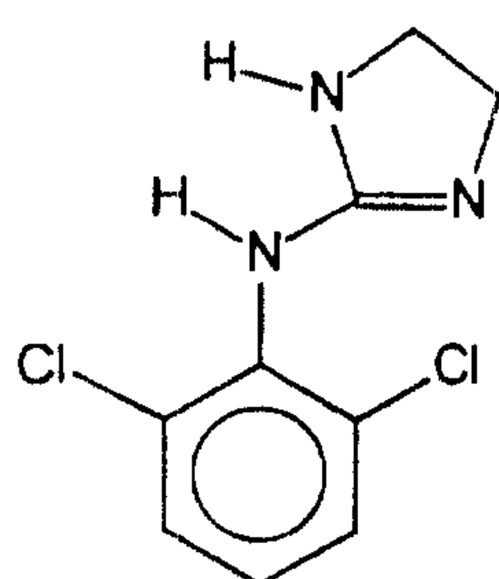
Alinidine
