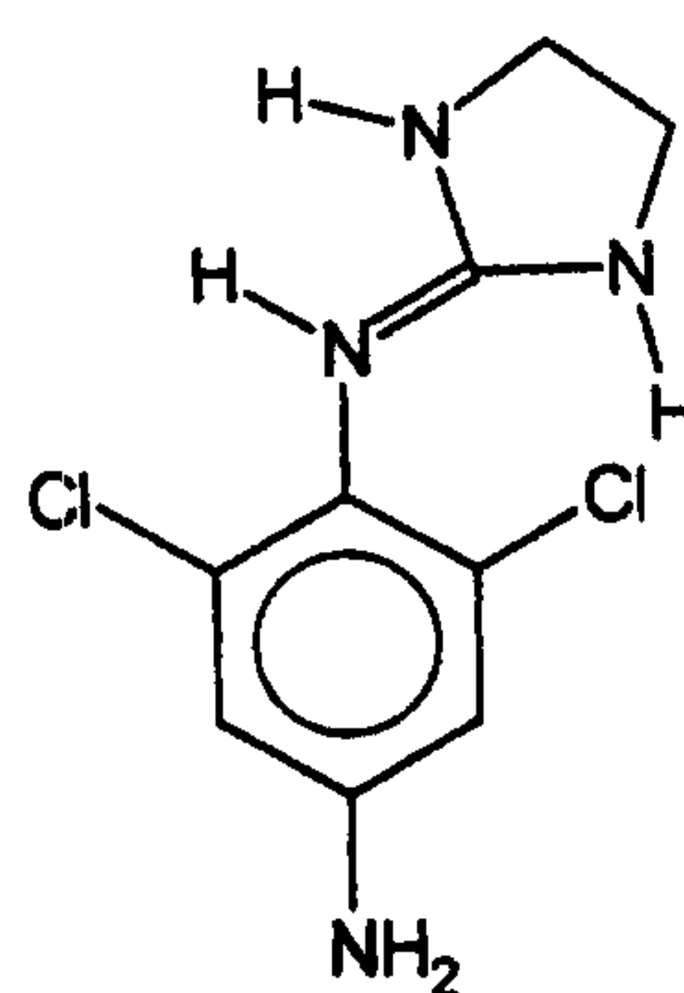
iopidine
