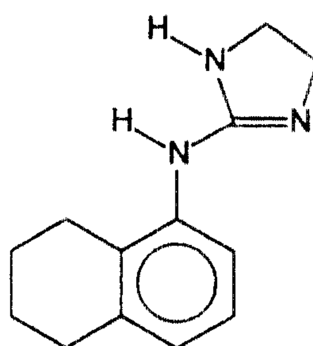
Tramazoline
