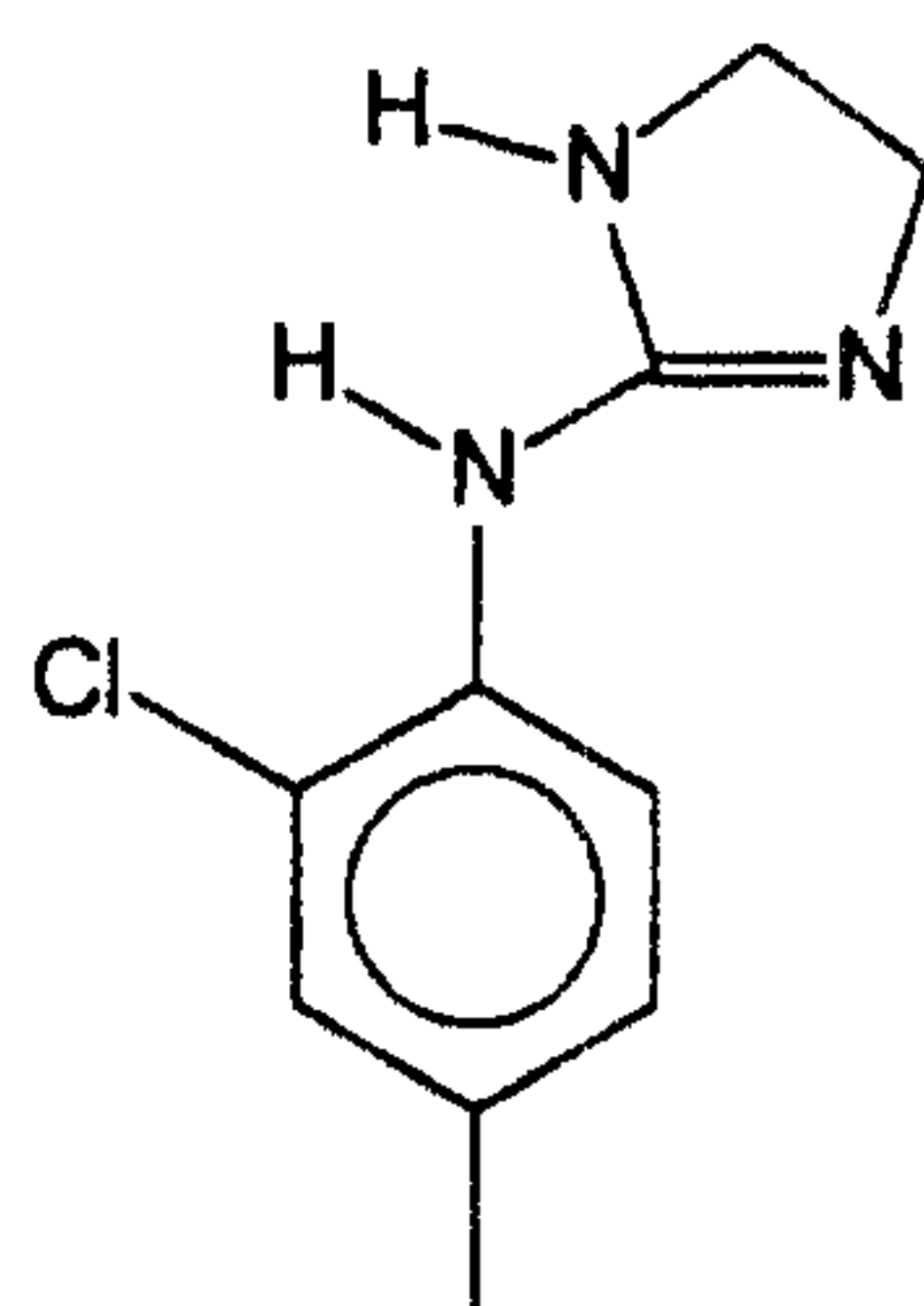
Tolonidine
