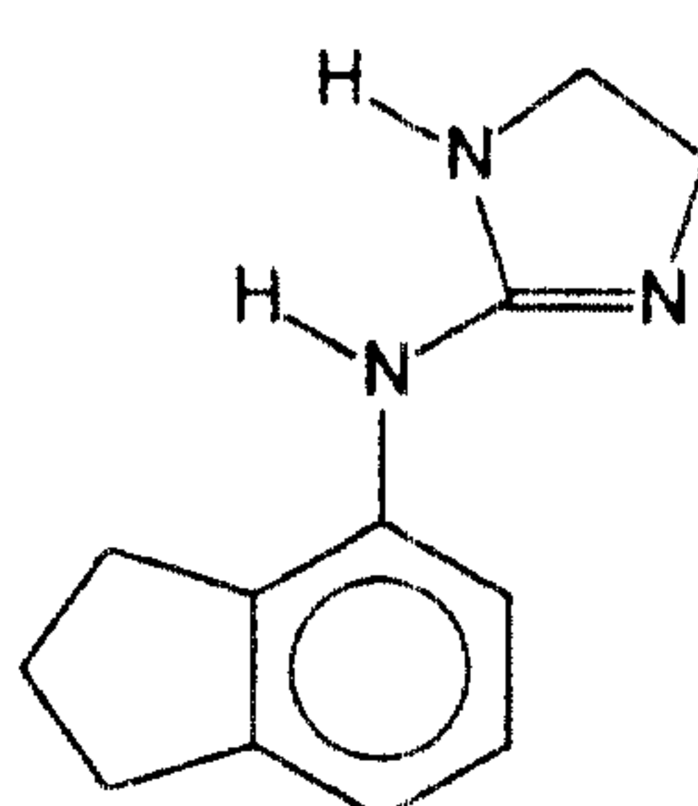
Iopidine
