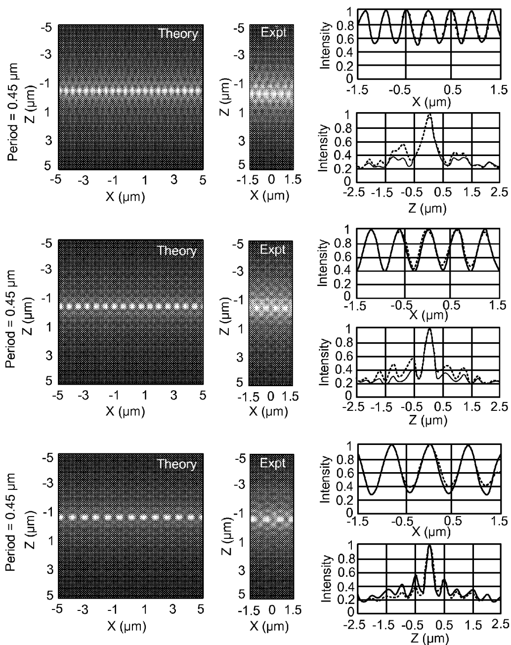
SI excitation pattern
