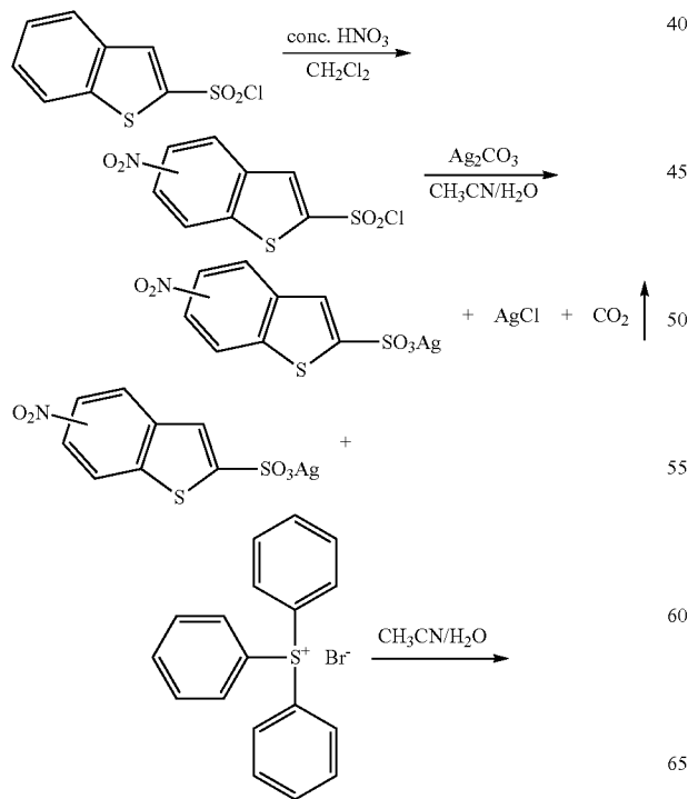
Scheme 1. Synthesis of fluorine-free fused-ring heteroaromatic PAGs.
