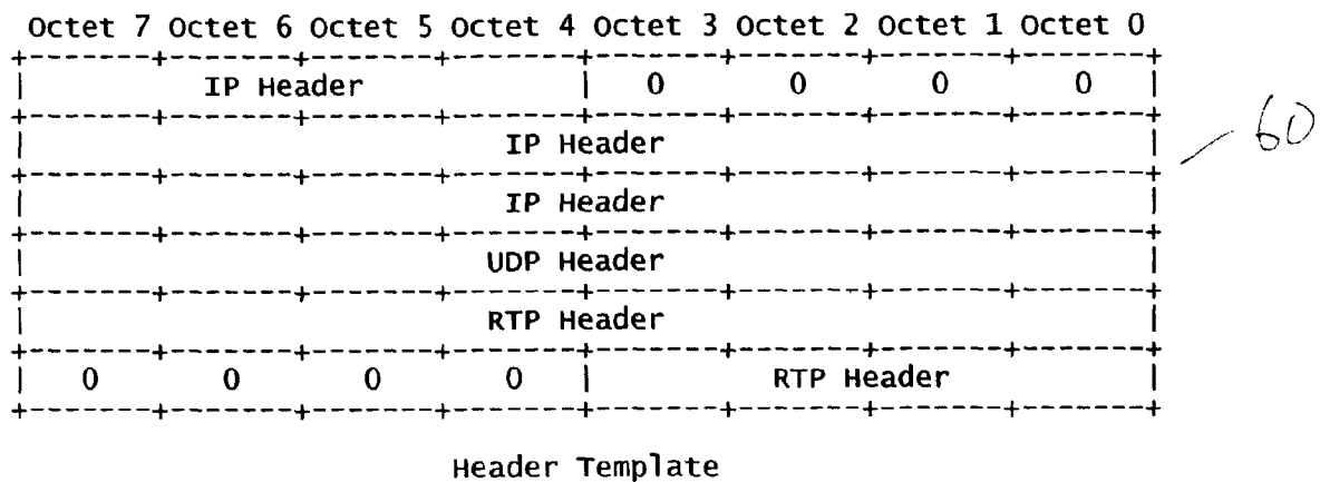
Egress Packet Buffer and Header Template
