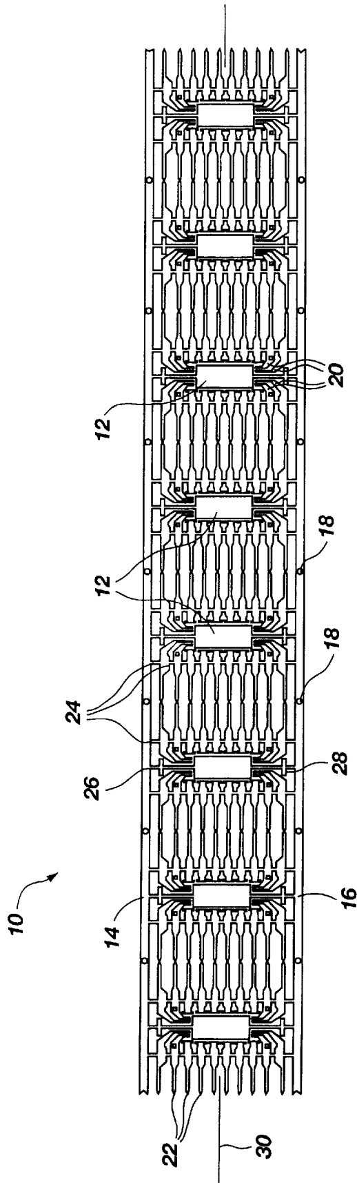
Fig. 1 (PRIOR ART)
