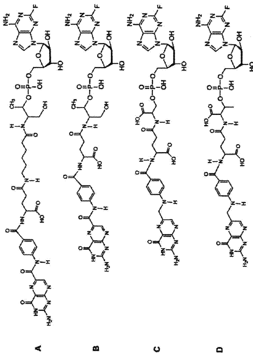
Figure 6: Fludarabine-Folate conjugates
