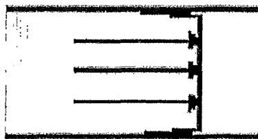
Electroosmotic flow
