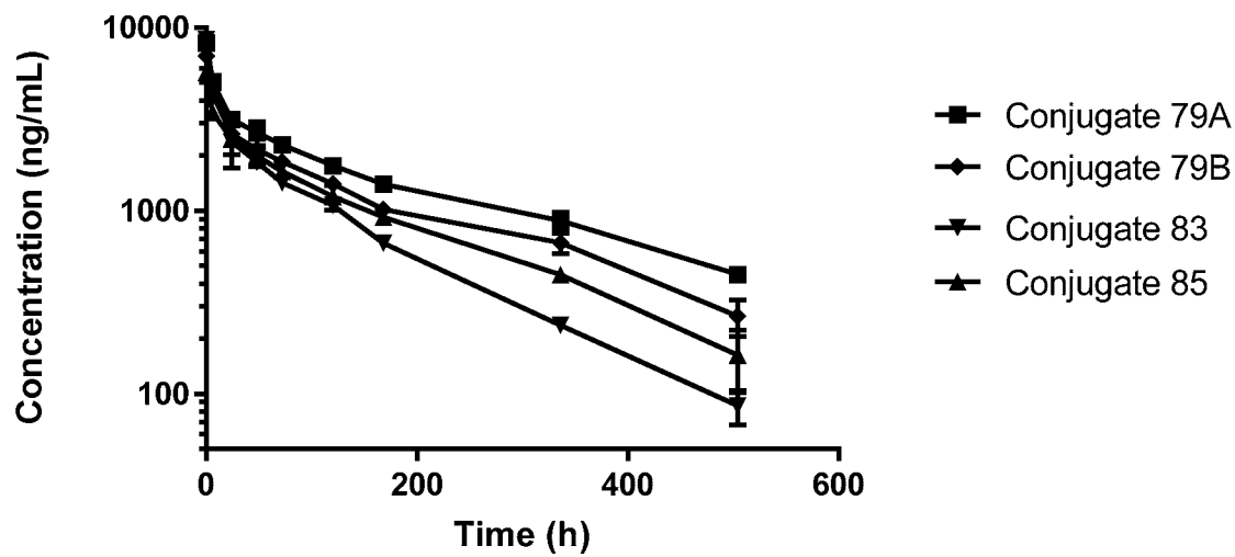
Figure 7C Conjugated AF-HPA
