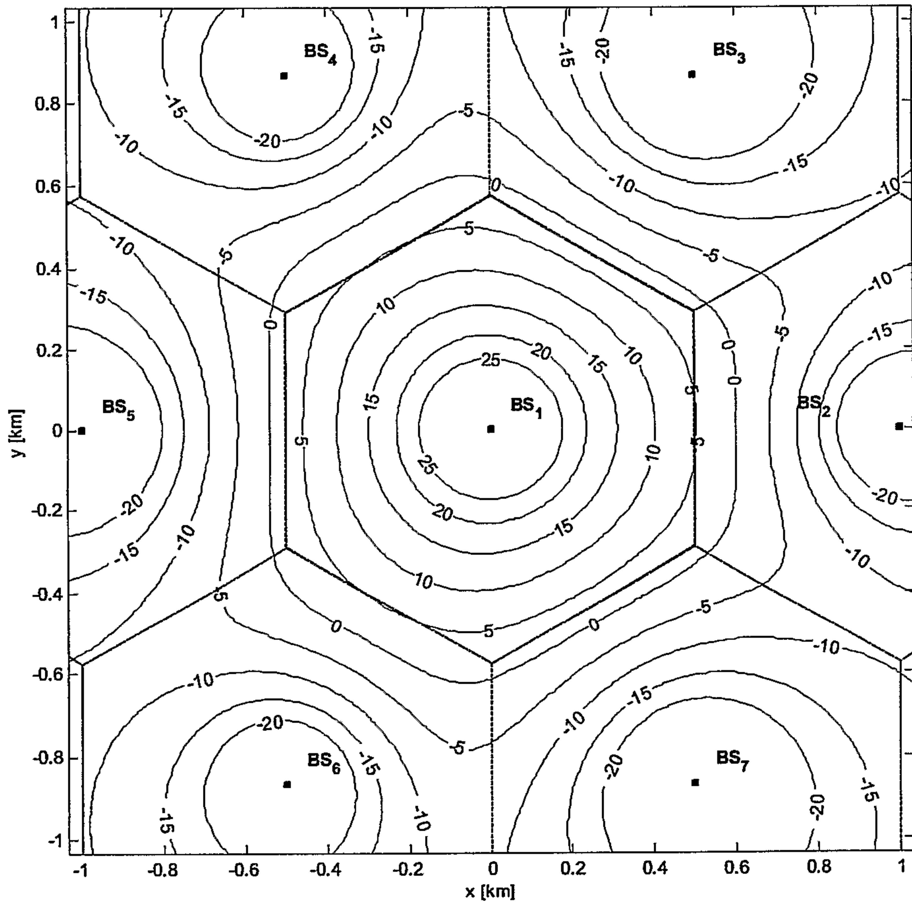
Subcarrier-Block-Set 1 (Power-Offset = 2.6 dB): SIR [dB] for BS 1
