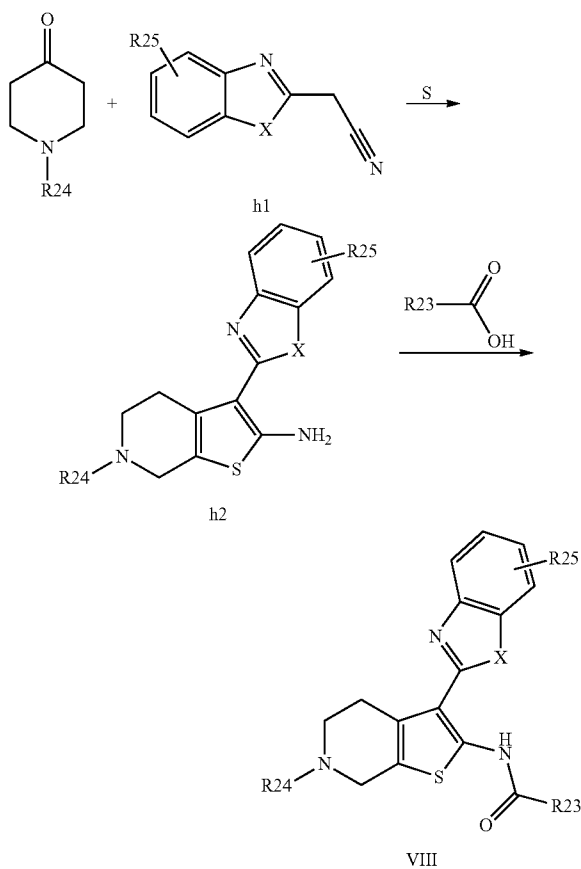
Scheme 8
