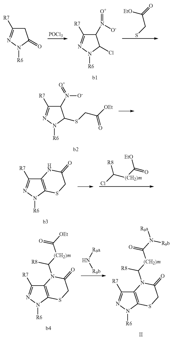
Scheme 2
