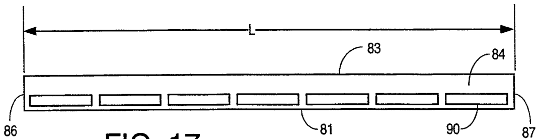
FIG. 17 (PRIOR ART)
