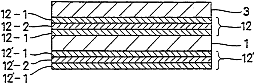
Fig. 5 (Prior Art)
