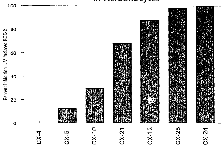
FIGURE 12A Percent Inhibition of UV Induced PGE-2 in Keratinocytes
