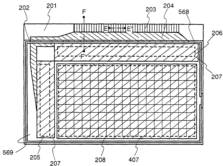
FIG. 7A top view
