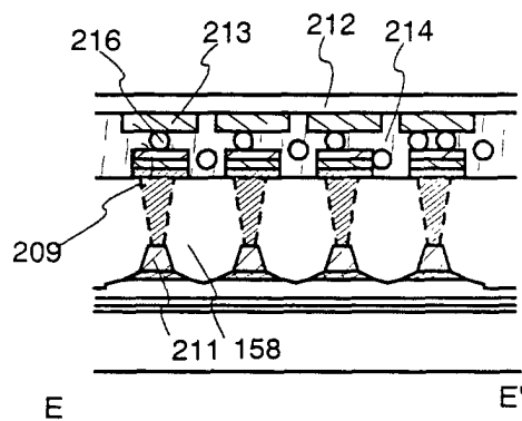
FIG. 7B cross sectional view of E-E'
