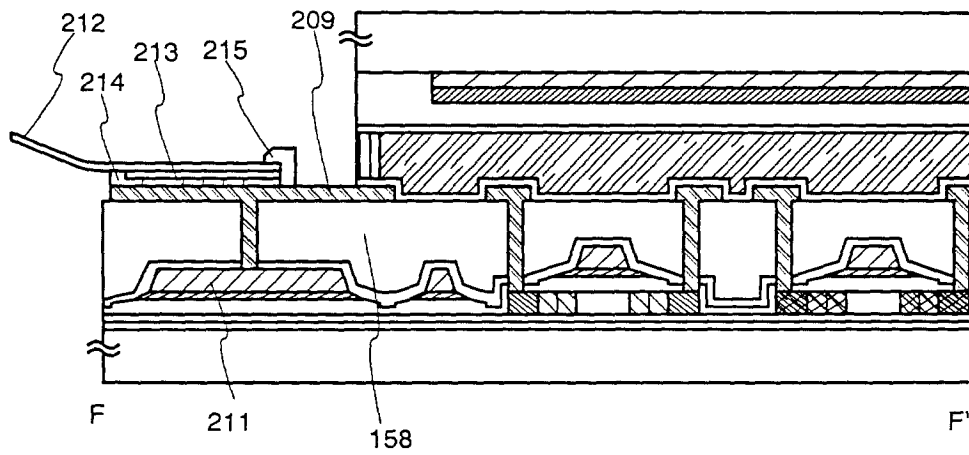
FIG. 8A cross sectional view of F-F'
