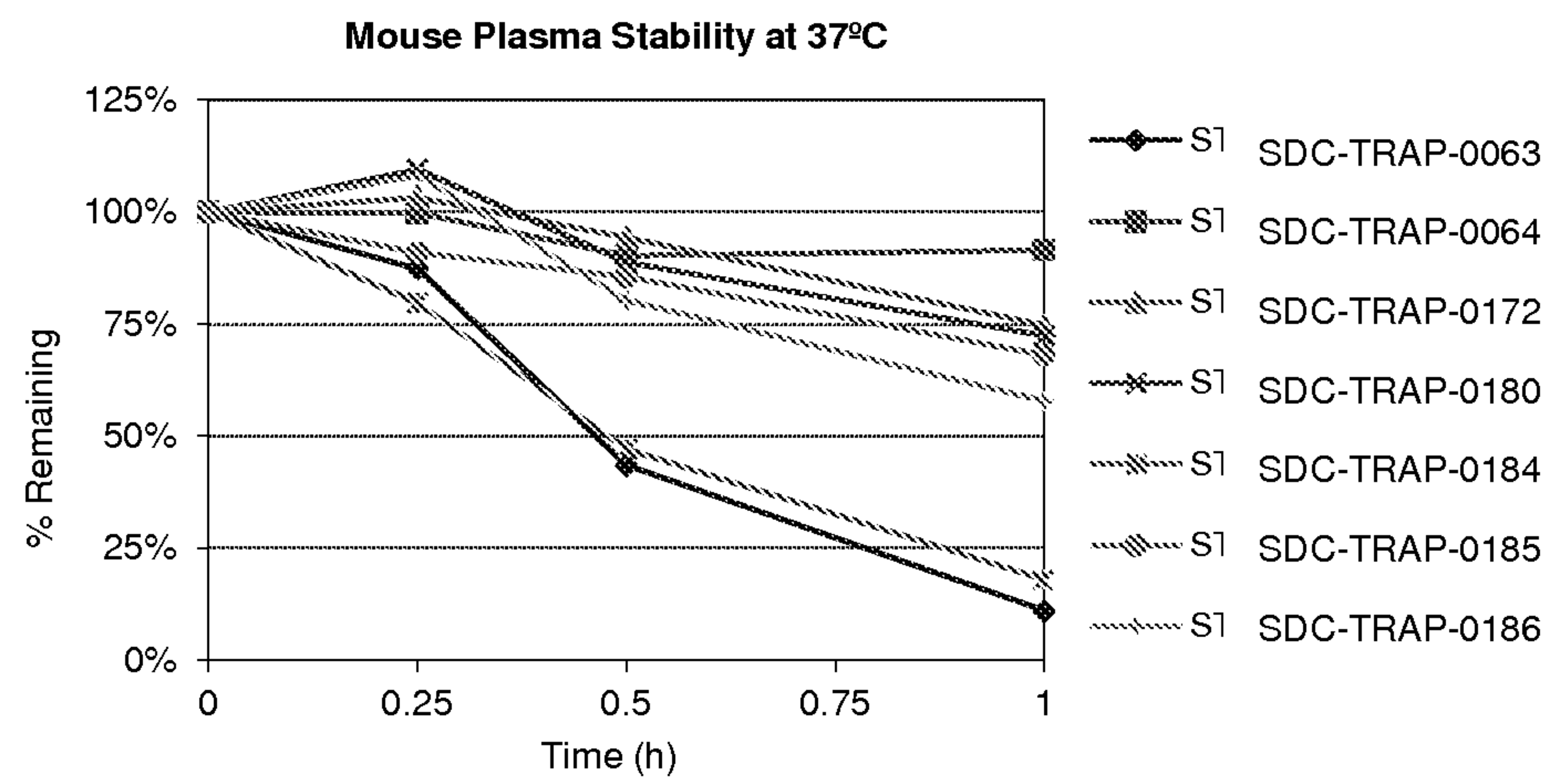
FIG 12: SDC-TRAP Stability in Mouse Plasma
