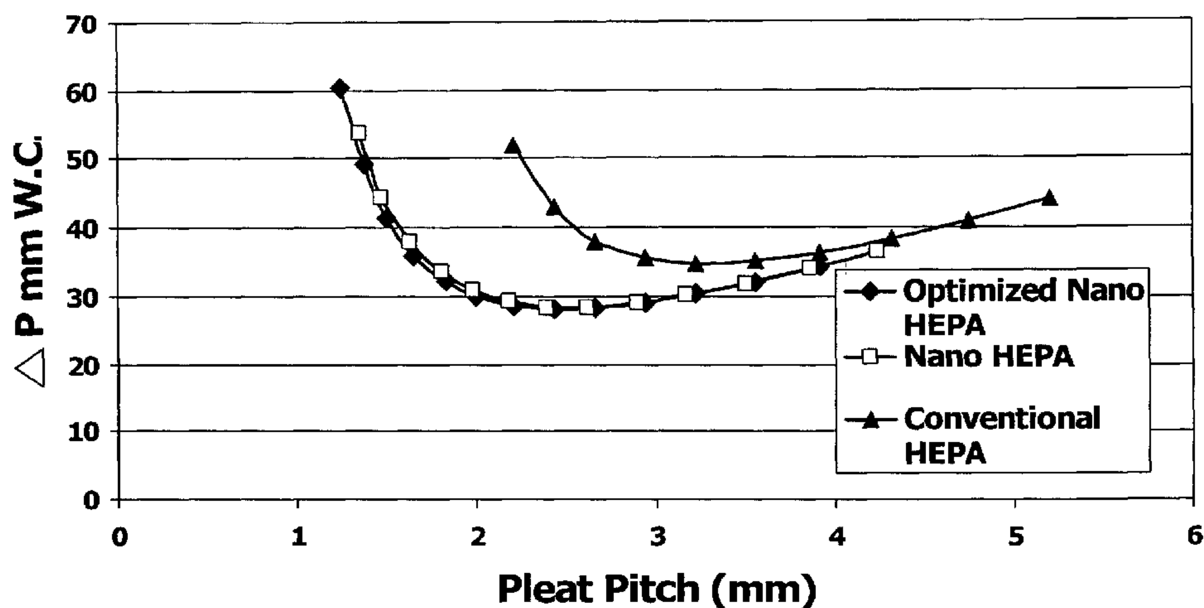
△ P of Water Column (mm W.C.) vs. Pleat Pitch
