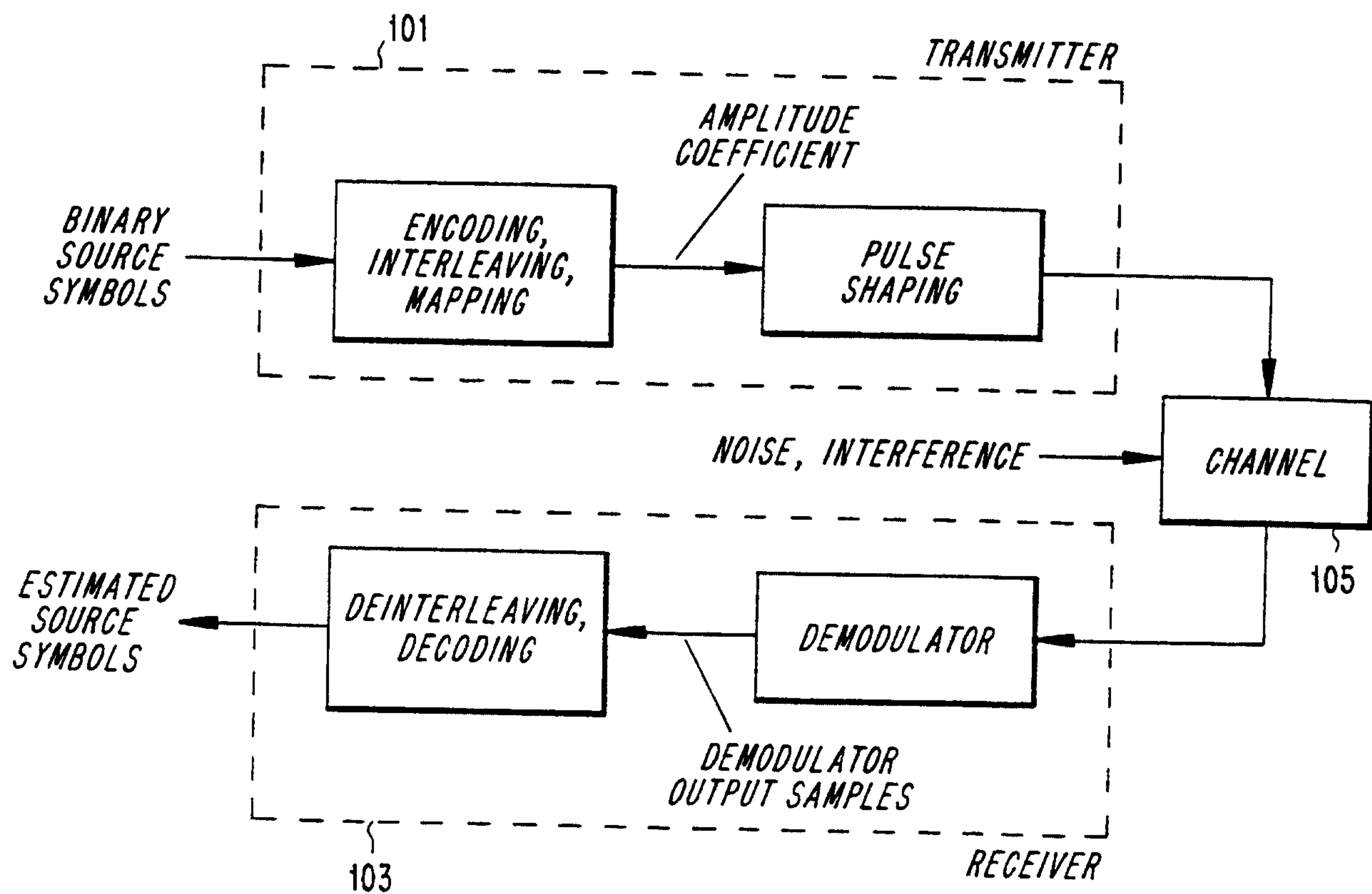
FIG. 1 (PRIOR ART)
