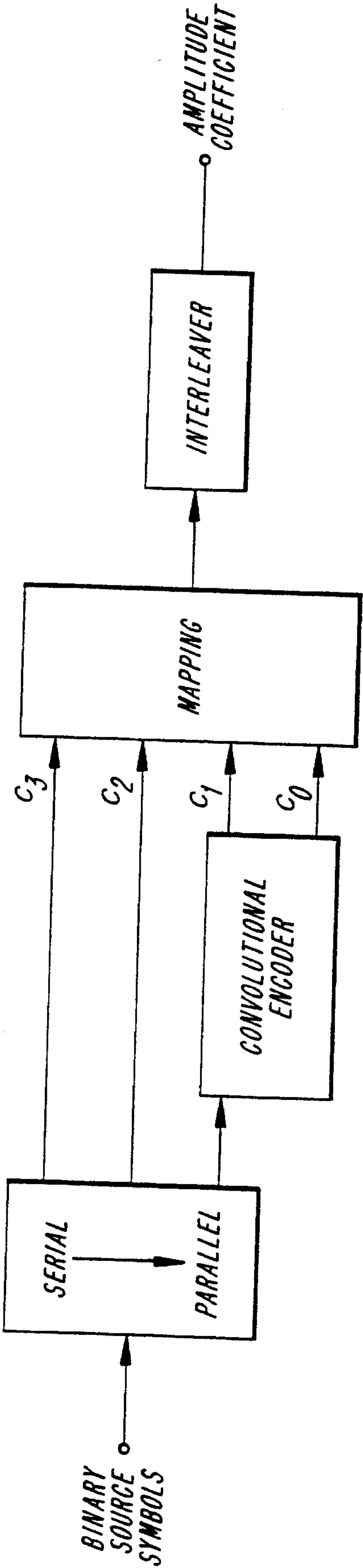
FIG. 5 (PRIOR ART)
