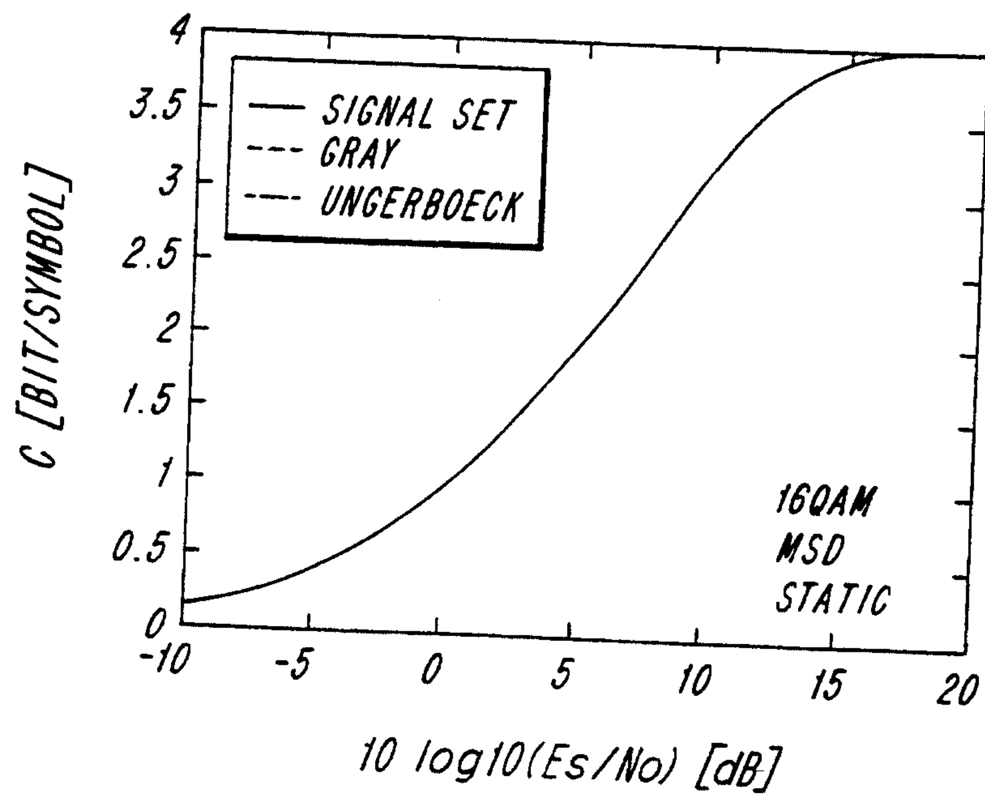
FIG. 12 (PRIOR ART)
