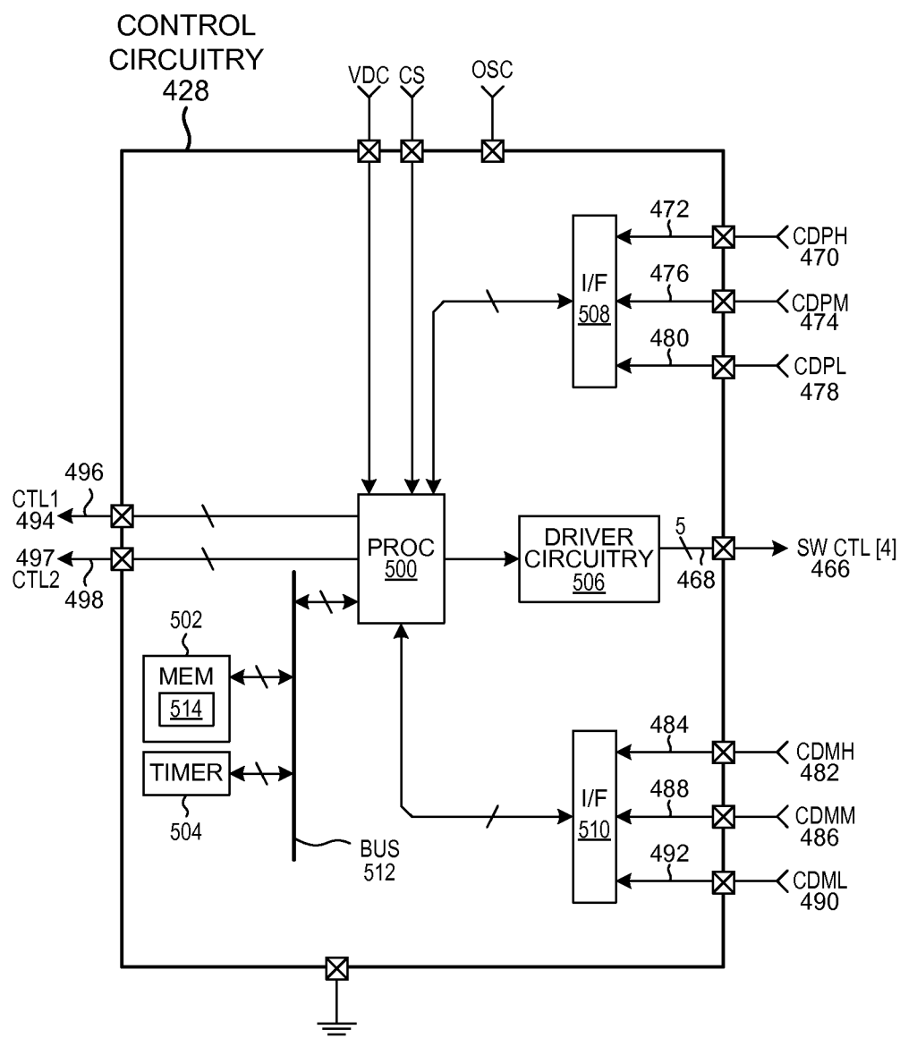
CONTROL CIRCUITRY
