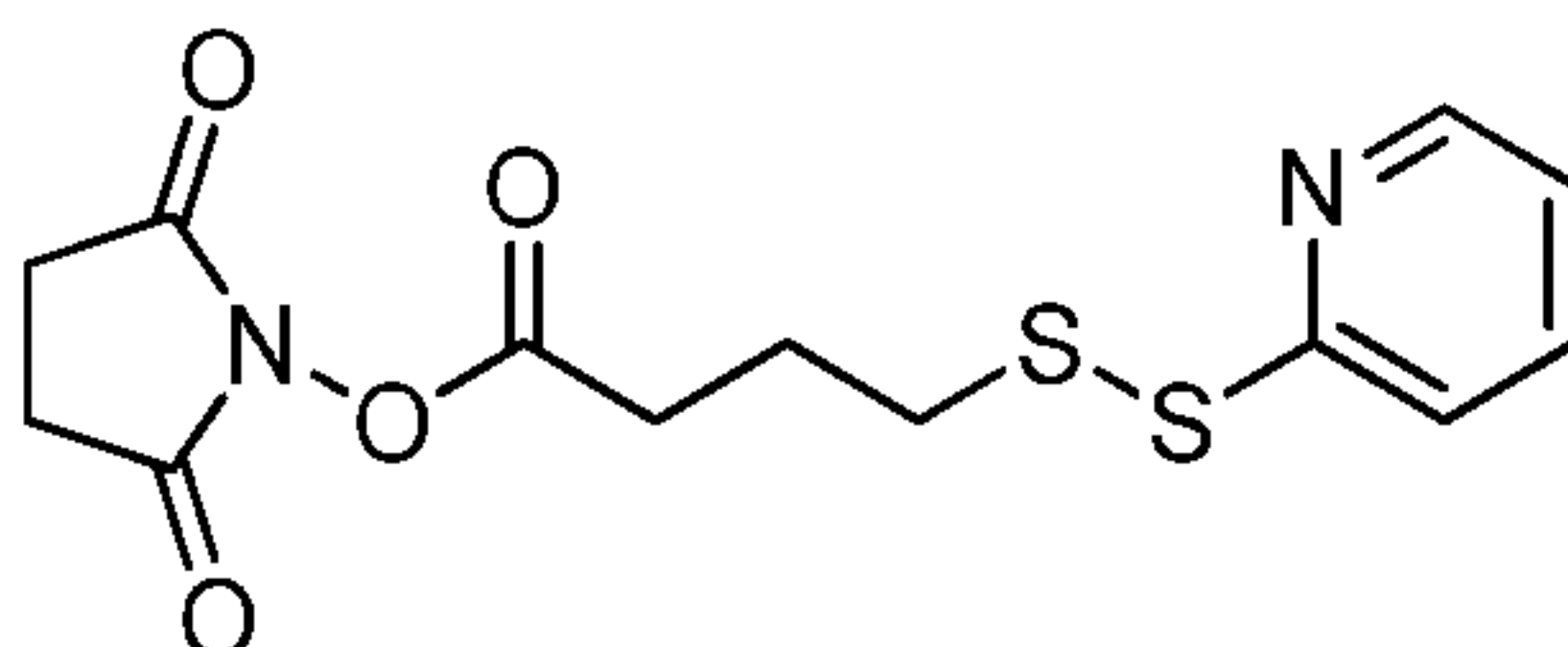
N-succinimidyl-4-(2-pyridyldithio)butanoate (SPDB) and
