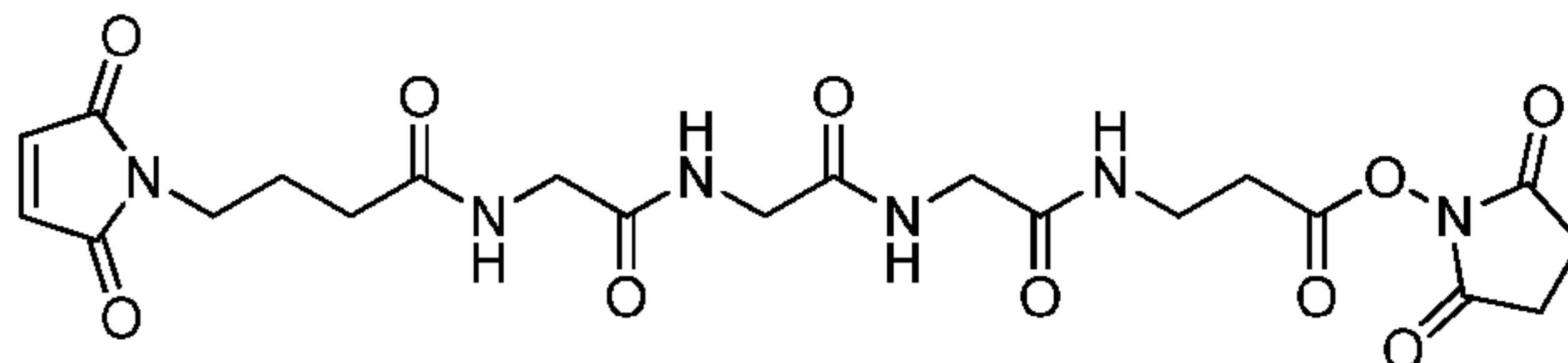
2,5-dioxopyrrolidin-1-yl 17-(2,5-dioxo-2,5-dihydro-1H-pyrrol-1-yl)-5,8,11,14-tetraoxo-4,7,10,13-tetraazaheptadecan-1-oate (CX1-1)
