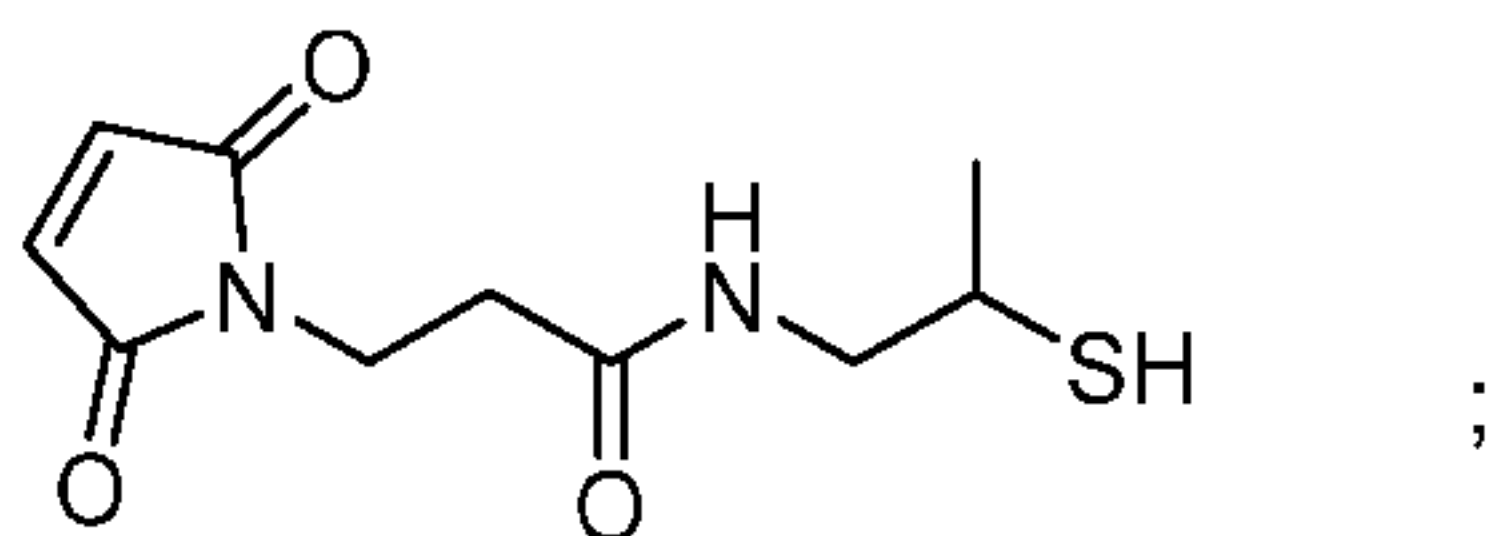
MPPT: MaleimidoPropionamidoPropaneThio
