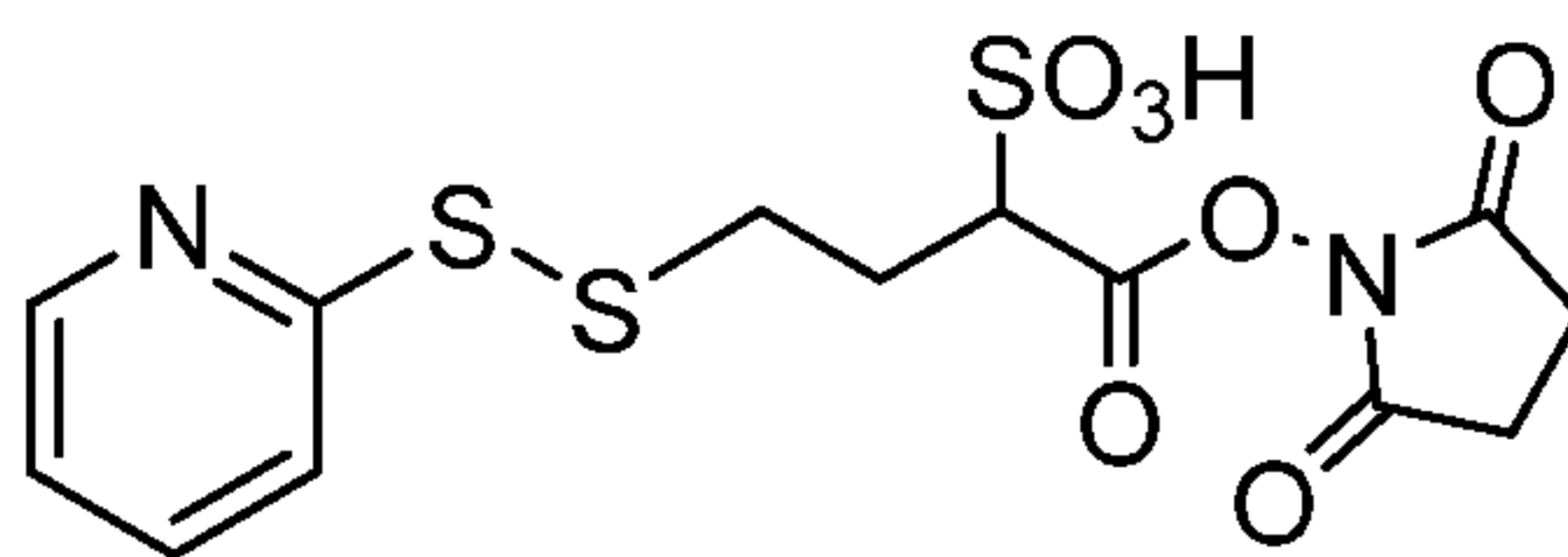
N -succinimidyl-4-(2-pyridyldithio)-2-sulfo-butanoate (sulfo-SPDB).
