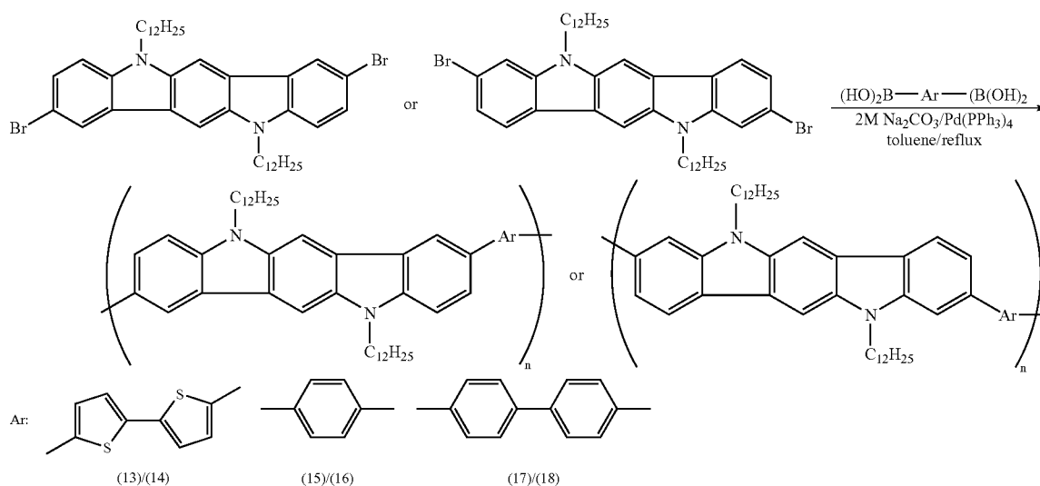
Scheme 3. Synthesis of Polymer (13).
