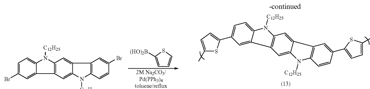
Scheme 3. Synthesis of Polymer (13).
