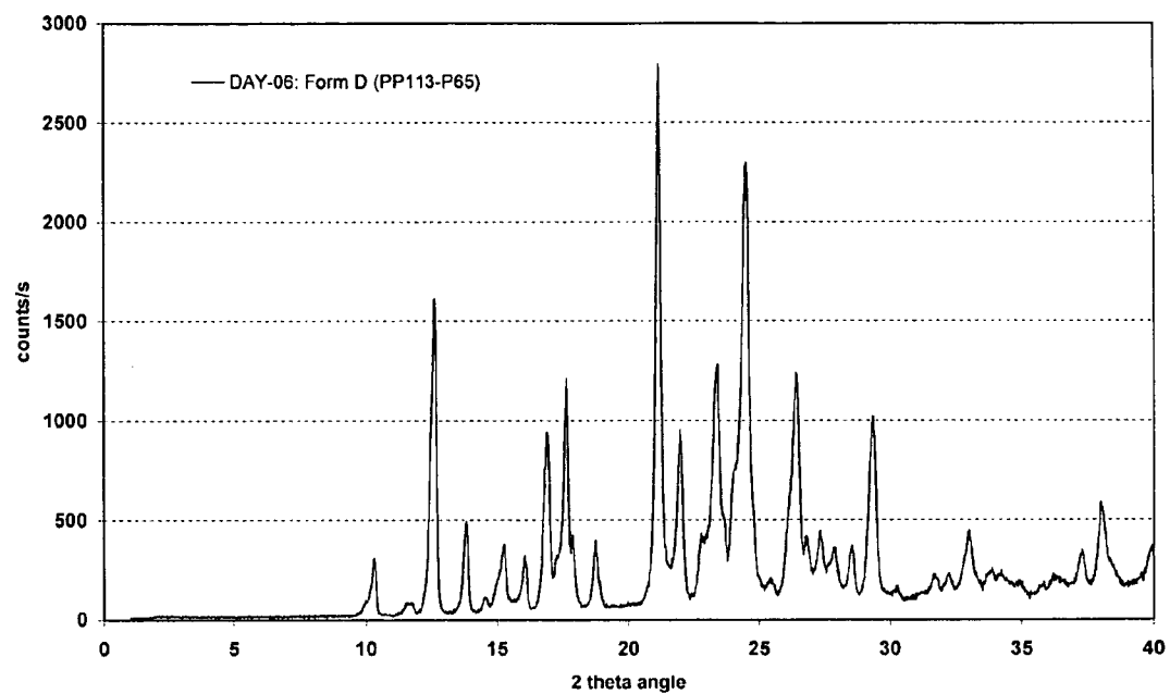
Figure 4 (N-desmethylozapine Form D)
