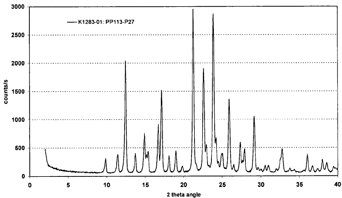
Figure 2 (N-desmethyloclozapine Form B)
