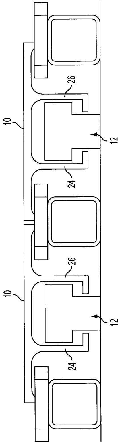
FIG. 1 PRIOR ART
