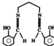
1,3-disalicylidene propanediamine
