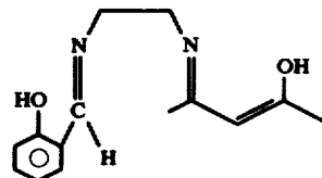
N-(4-hydroxyl-2-pent-3-enylidene)-N'-salicylidene-1,2-ethanediamine (average structure)
