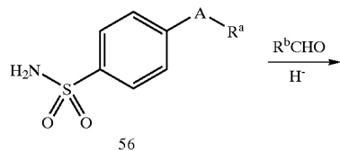
Scheme XX
