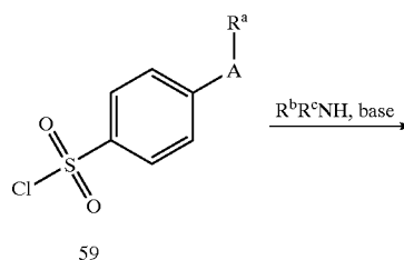
Scheme XIII
