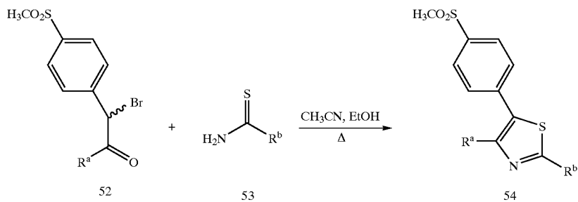
Scheme X
