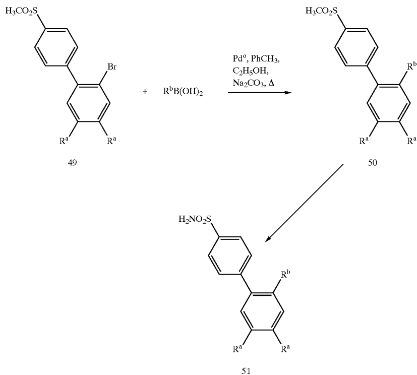
Scheme IX
