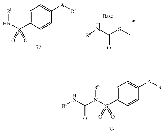
Scheme XXI
