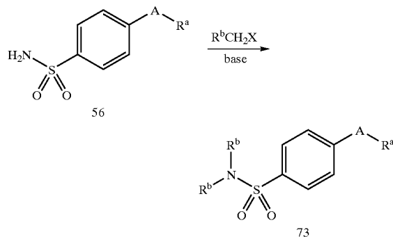
Scheme XIX
