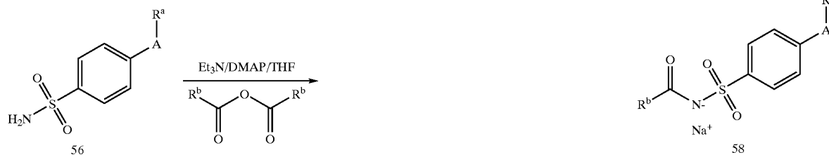
Scheme XI
