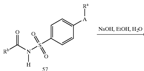
Scheme XII
