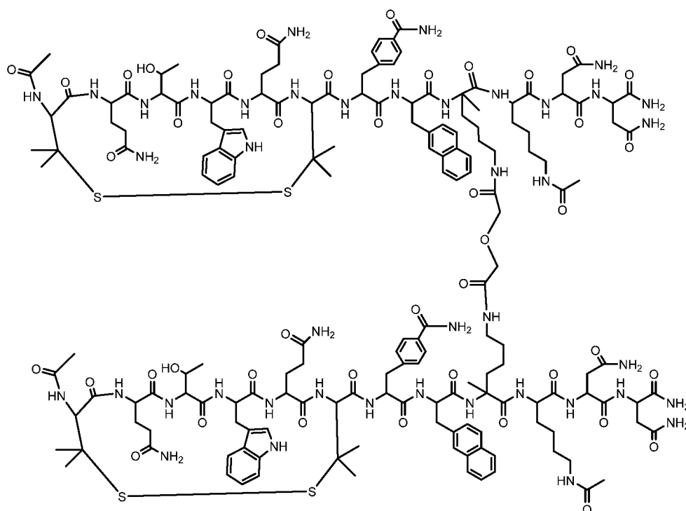
Compound D
