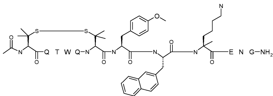
Compound B
