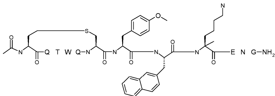
Compound A
