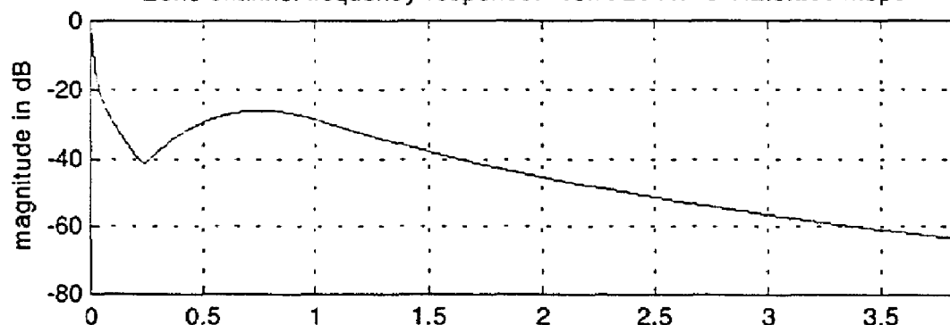
Echo channel frequency response. 15kft 26 AWG Rate:2304kbps
