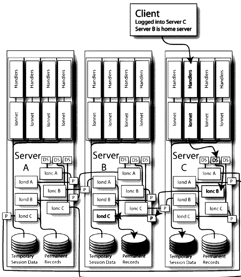
Fig. 2A – Overview of Network Communication
