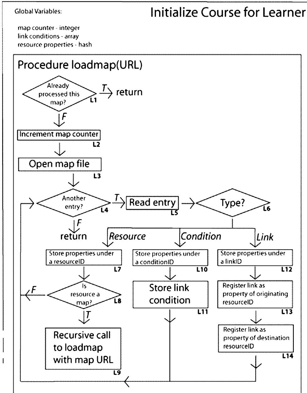
Fig. 9A – Flow chart of procedure loadmap
