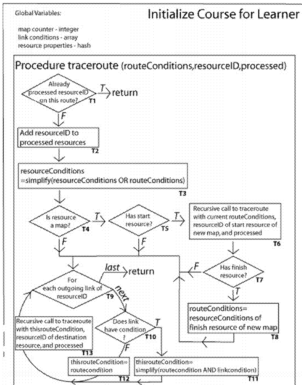
Fig. 11A – Flow chart of procedure traceroute
