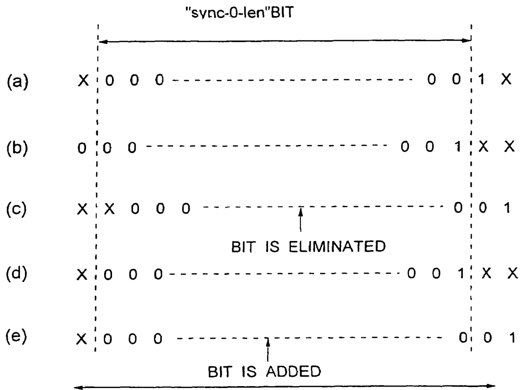
SYNCHRONIZATION CODE DETECTION WINDOW OF "sync-0-len+2"BIT
