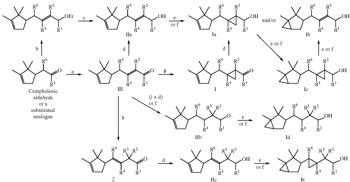
Scheme 1 Access to cyclopropanated campholenic aldehyde derivatives Ia-e
