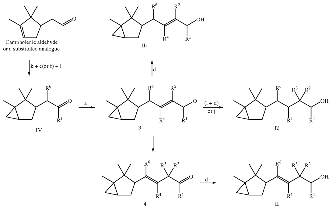
Scheme 2 Access to cyclopropanated campholenic aldehyde derivatives Ib, d, f
