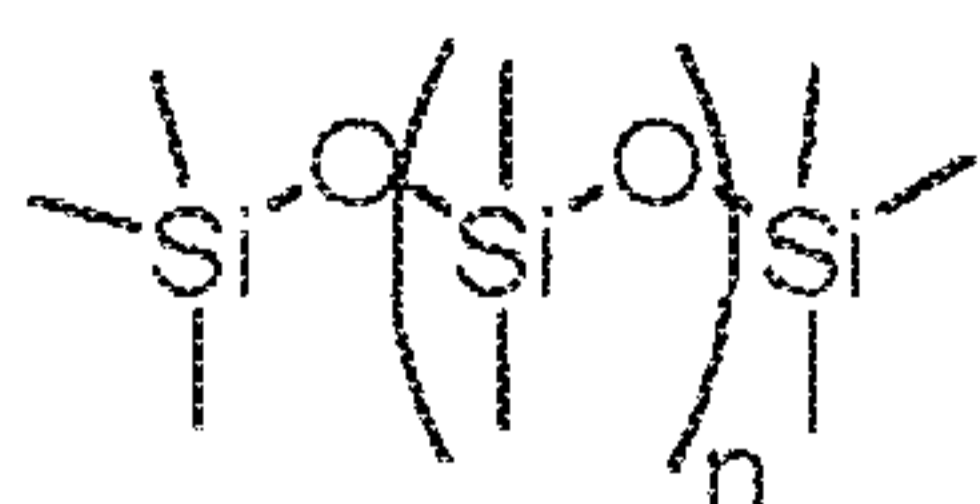
Polydimethylsiloxane
