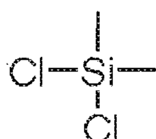
Dimethyldichlorosilane
