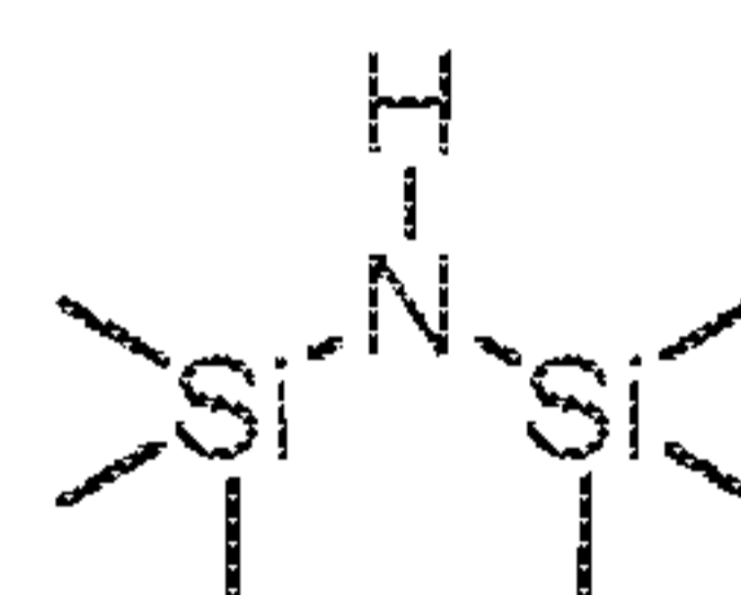
Hexamethyldisilazane
