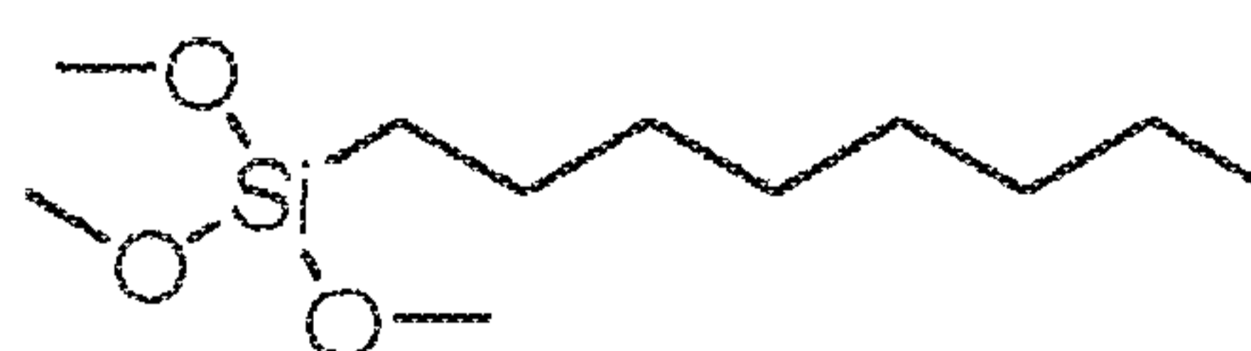
Octyltrimethoxysilane
