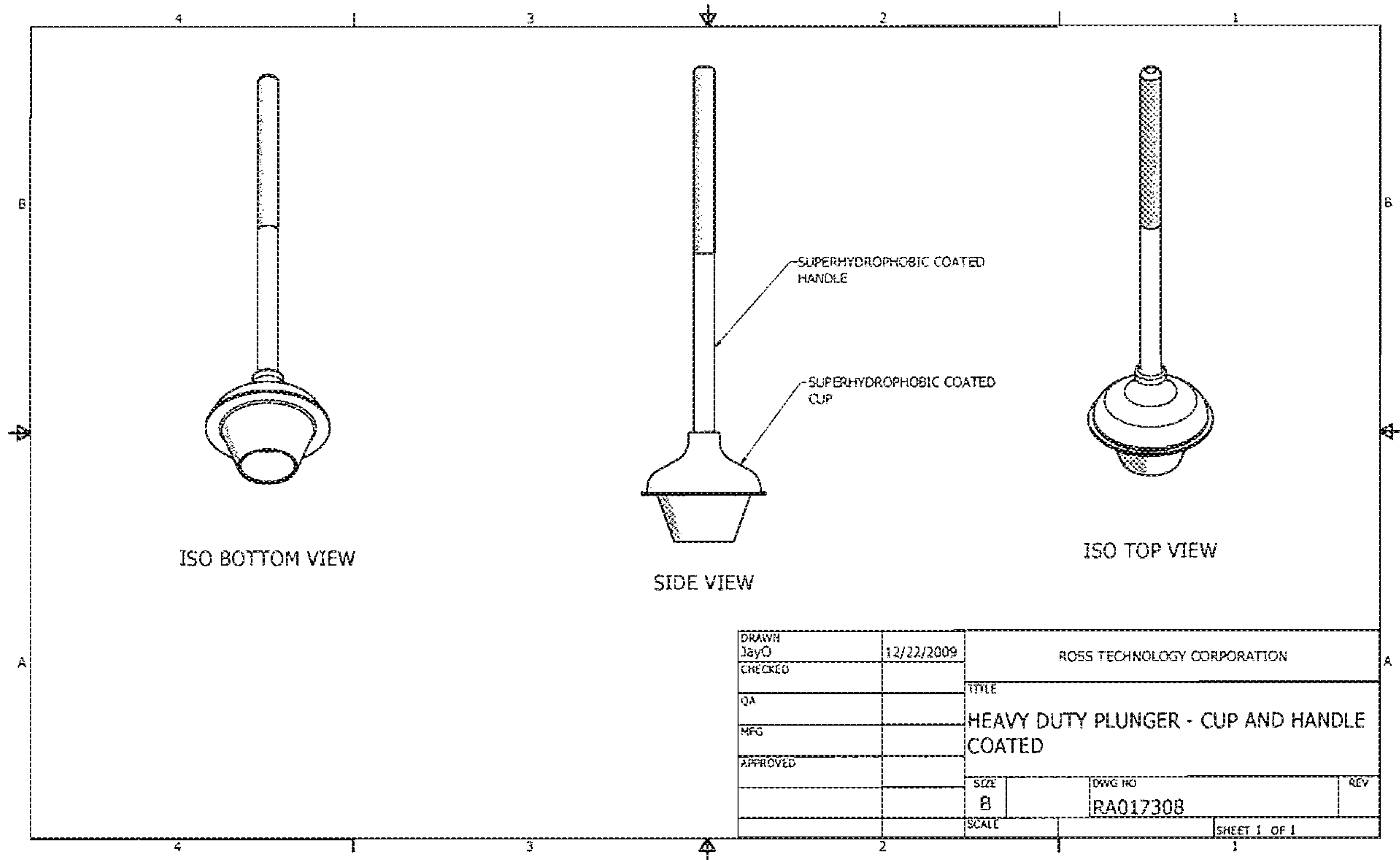
Figure 5: Coated cup and handle – industrial plunger.
