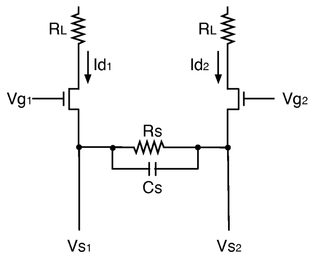
FIG. 1C (PRIOR ART)
