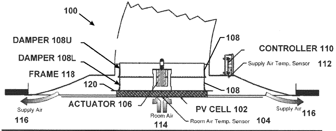
Figure 1: SVAV diffuser cross-section
