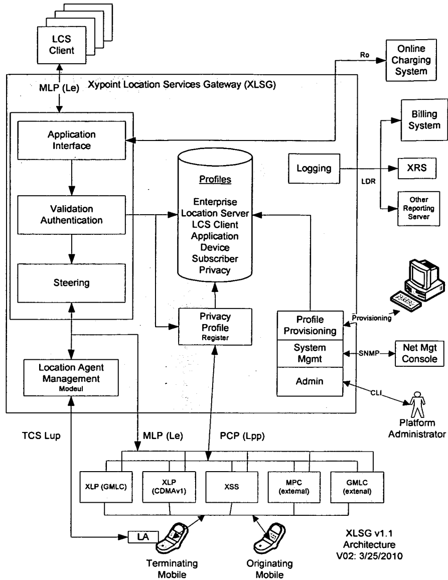
XLSG v1.1 Architecture
