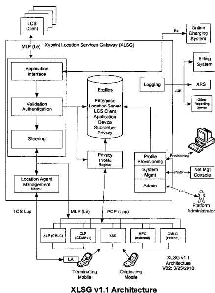
XLSG v1.1 Architecture
