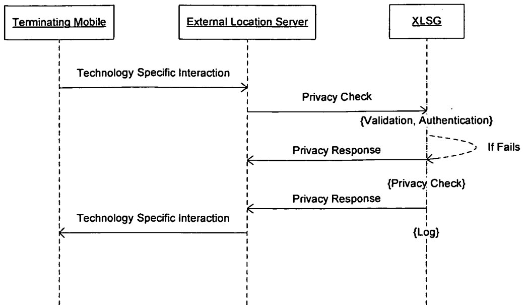
Authorization Request Message Flow
