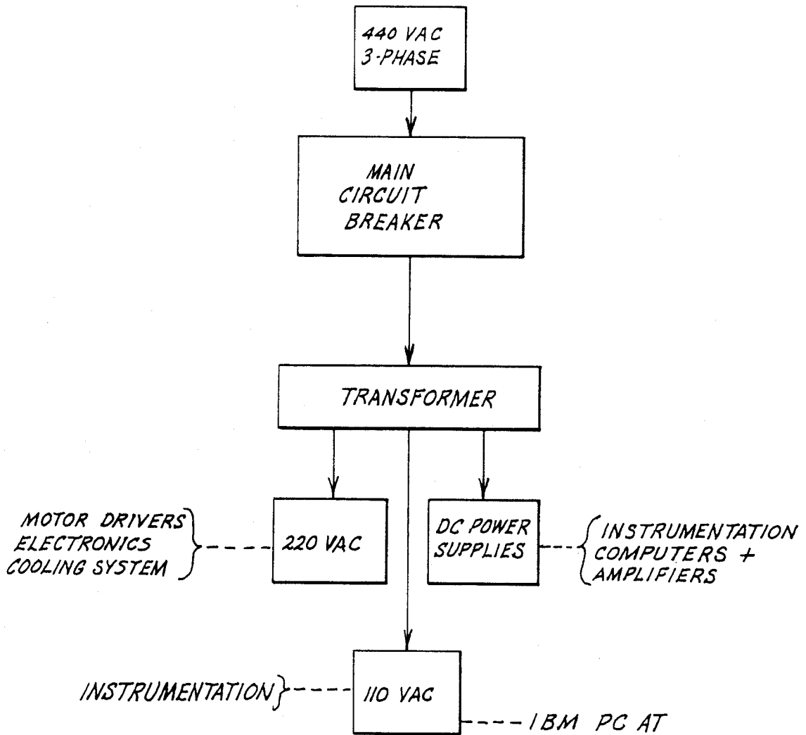
POWER DISTRIBUTION
