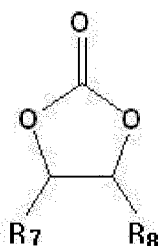
[Chemical Formula 2]
