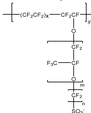
[Chemical Formula 1]
