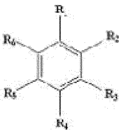
[Chemical Formula 1]
