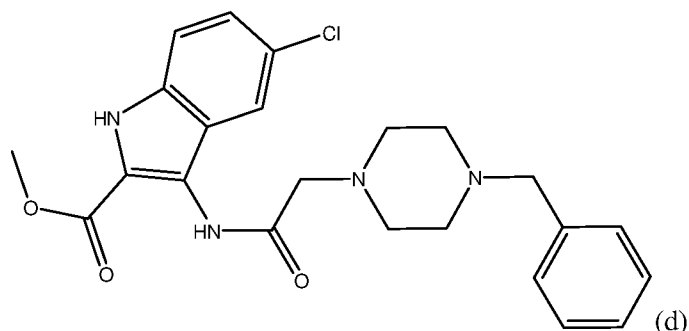
3-[2-(4-Benzyl-piperazin-1-yl)-acetylamino]-5-chloro-1 H -indole-2-carboxylic acid methyl ester
