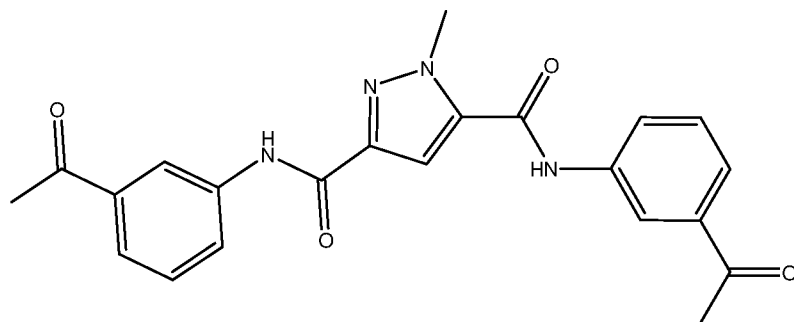
1-Methyl-1 H -pyrazole-3,5-dicarboxylic acid bis-[(3-acetyl-phenyl)-amide]
