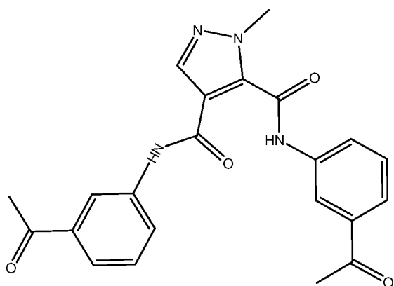
2-Methyl-2 H -pyrazole-3,4-dicarboxylic acid bis-[(3-acetyl-phenyl)-amide]
