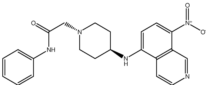
2-[4-(8-Nitro-isoquinolin-5-ylamino)-piperazin-1-yl]-N-phenyl-acetamide
