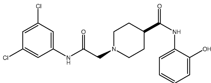
1-[(3,5-Dichloro-phenylcarbamoyl)-methyl]-piperidine-4-carboxylic acid (2-hydroxy-phenyl)-amide
