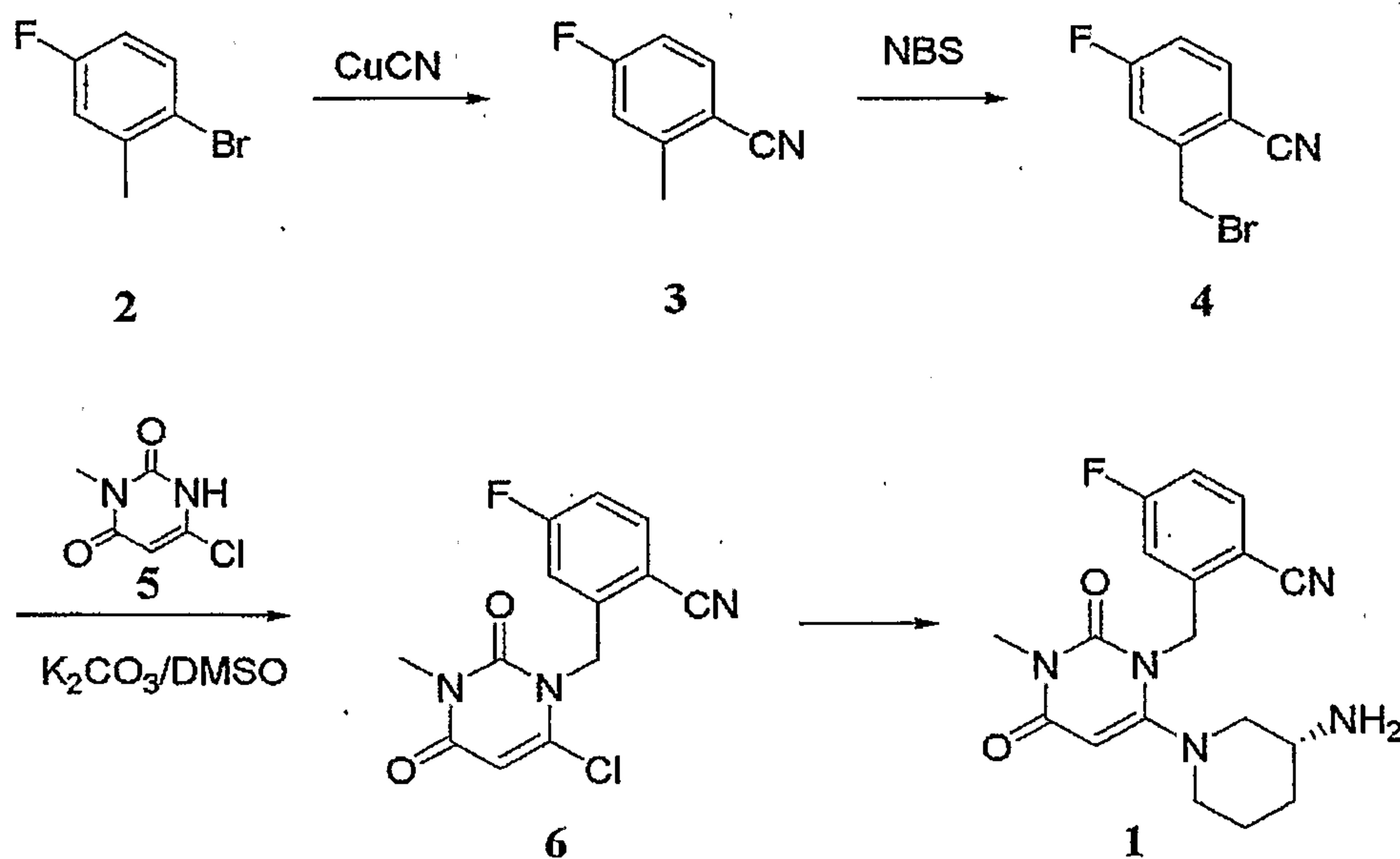
4-Fluoro-2-methylbenzonitrile (3)
