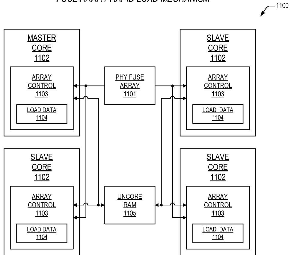
FUSE ARRAY RAPID LOAD MECHANISM
