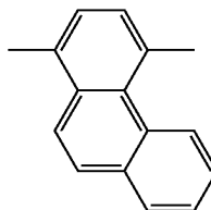
1,4-naphthylene
