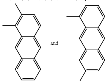
1,2- and 1,7-anthrylenes
