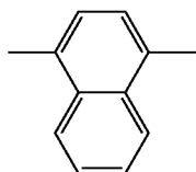
1,4-naphthylene
