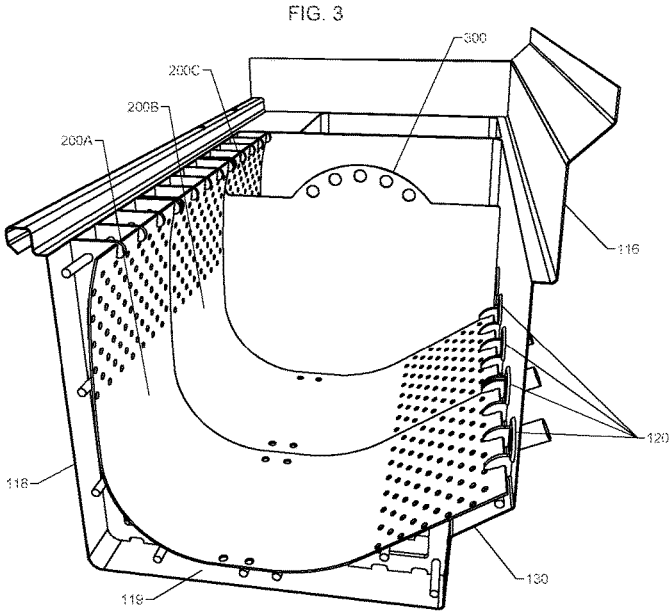
TRANSVERSE SECTION
