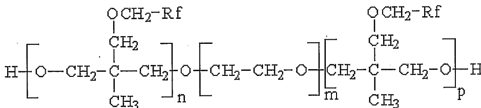
Structural Formula (19)
