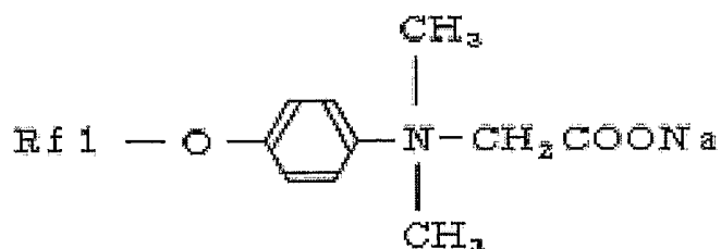
Structural Formula (18)
