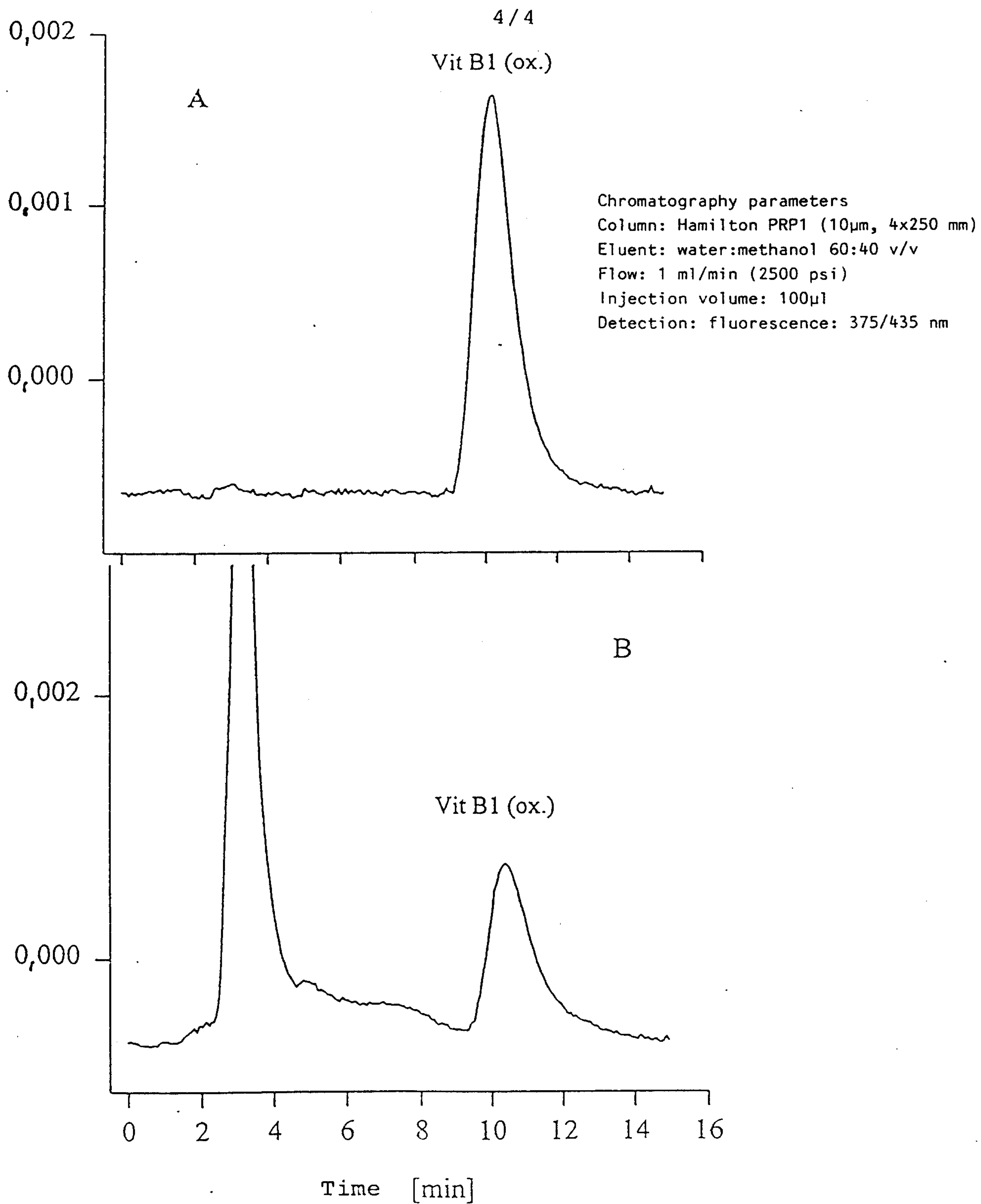
Chromatograms of a standard solution (104 \mu g/g thiamin hydrochloride) and the sample B0S6 (Fenugreek embryos after 3 days of germination)
