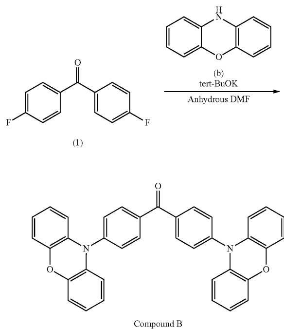
Compound B
