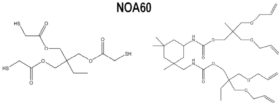
Trimethylolpropane Tris(2- mercaptoacetate)
