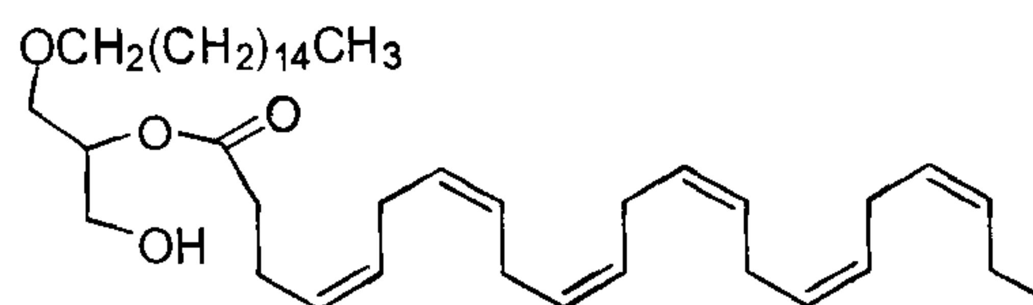
(4Z,7Z,10Z,13Z,16Z,19Z)-1-(hexadecyloxy)-3-hydroxypropan-2-yl docosa-4,7,10,13,16,19-hexaenoate
