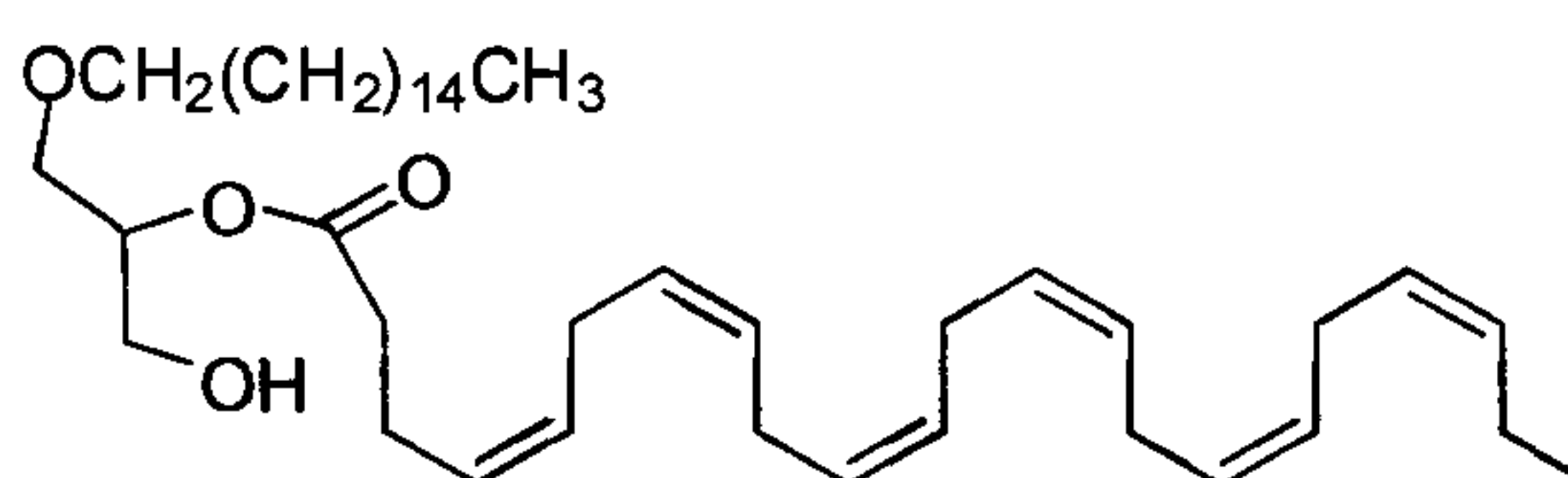
(4Z,7Z,10Z,13Z,16Z,19Z)-1-(hexadecyloxy)-3-hydroxypropan-2-yl docosa-4,7,10,13,16,19-hexaenoate
