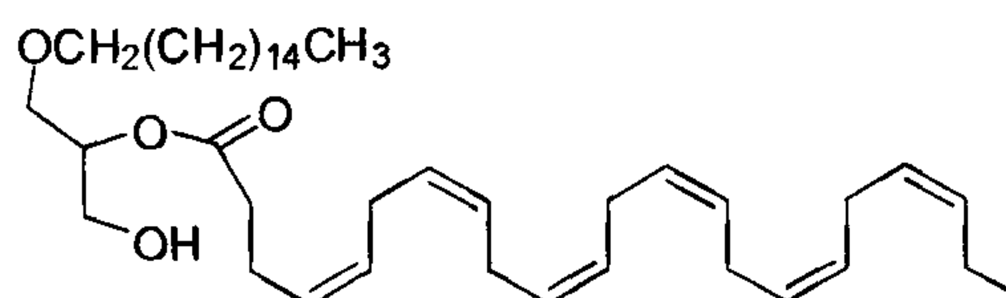
(4Z,7Z,10Z,13Z,16Z,19Z)-1-(hexadecyloxy)-3-hydroxypropan-2-yl docosa-4,7,10,13,16,19-hexaenoate
