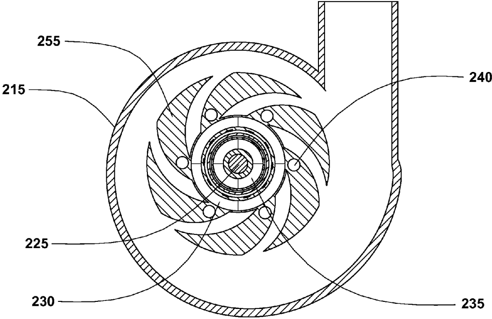
FIG. 19 (Section G-G)
