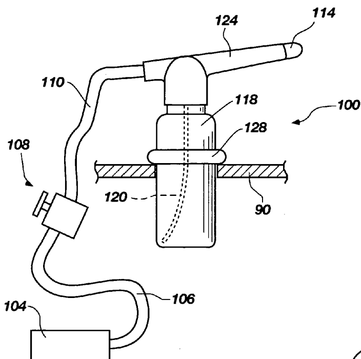
FIG. 4 (PRIOR ART)
