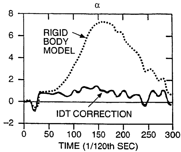
ORIENTATION (deg) FIG._17A
