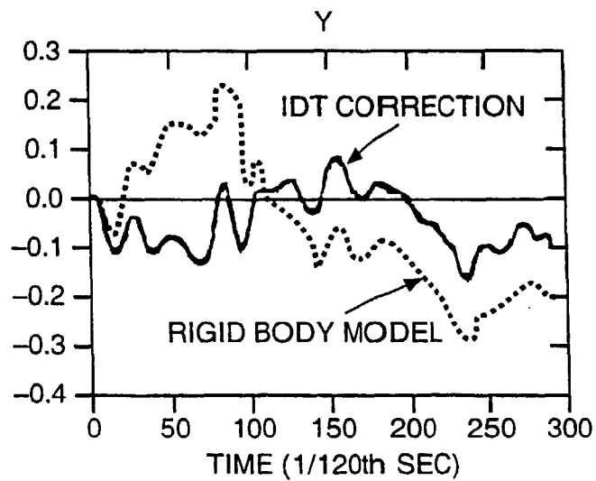
DISPLACEMENT (cm) FIG._ 16B
