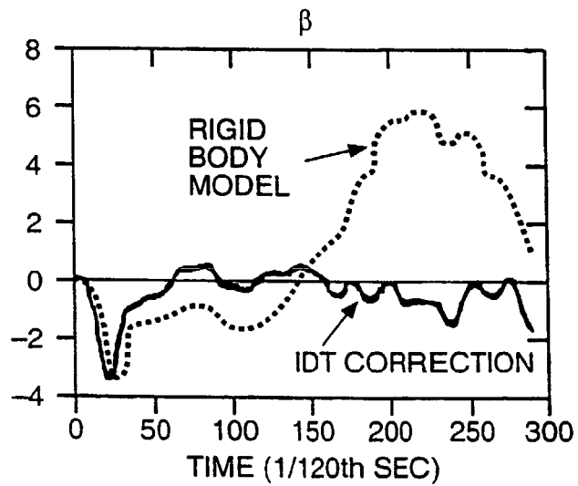
ORIENTATION (deg) FIG._17B
