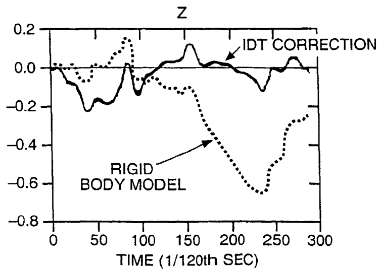
DISPLACEMENT (cm) FIG._ 16C
